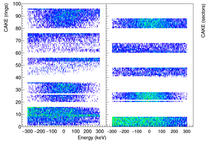
Figure 4.18: Left panel: Counts in the rings as a function of the energy difference between the sector and the ring pair. Right panel: Sector counts as a function of the energy difference between the sector and the ring pair.
