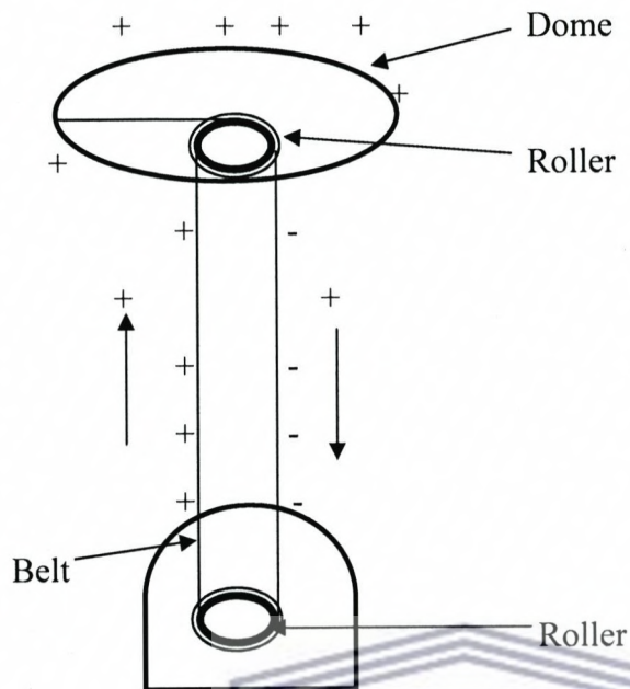
Figure 4.2: A Simple diagram of a Van de Graaff generator
