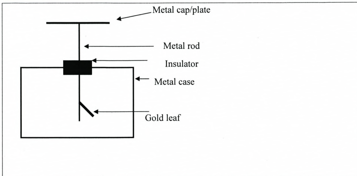
Figure 4.1: A simple diagram of a gold-leaf electroscope
