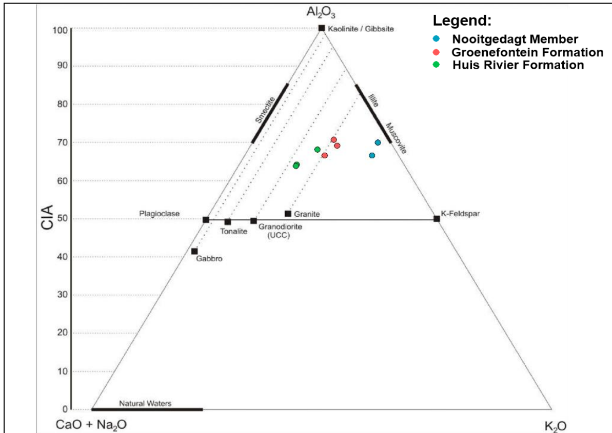
Figure 4-10: CIA diagram showing the general weathering trend of the sampled lithologies of the Cango Caves Group. Modified after Nesbitt and Young (1989).
