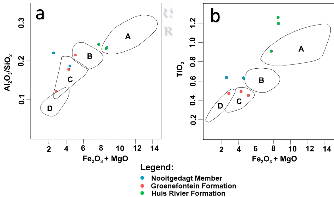
Figure 4-9: Major element composition plots of sands and sandstones for tectonic setting discrimination. a – \text{Al}_2\text{O}_3/\text{SiO}_2 vs \text{Fe}_2\text{O}_3 + \text{MgO} ; b – \text{TiO}_2 vs \text{Fe}_2\text{O}_3 + \text{MgO} , after Bhatia (1983). A = Oceanic Island Arc; B = Continental Island Arc; C = Active Continental Margin; D = Passive Margin.
