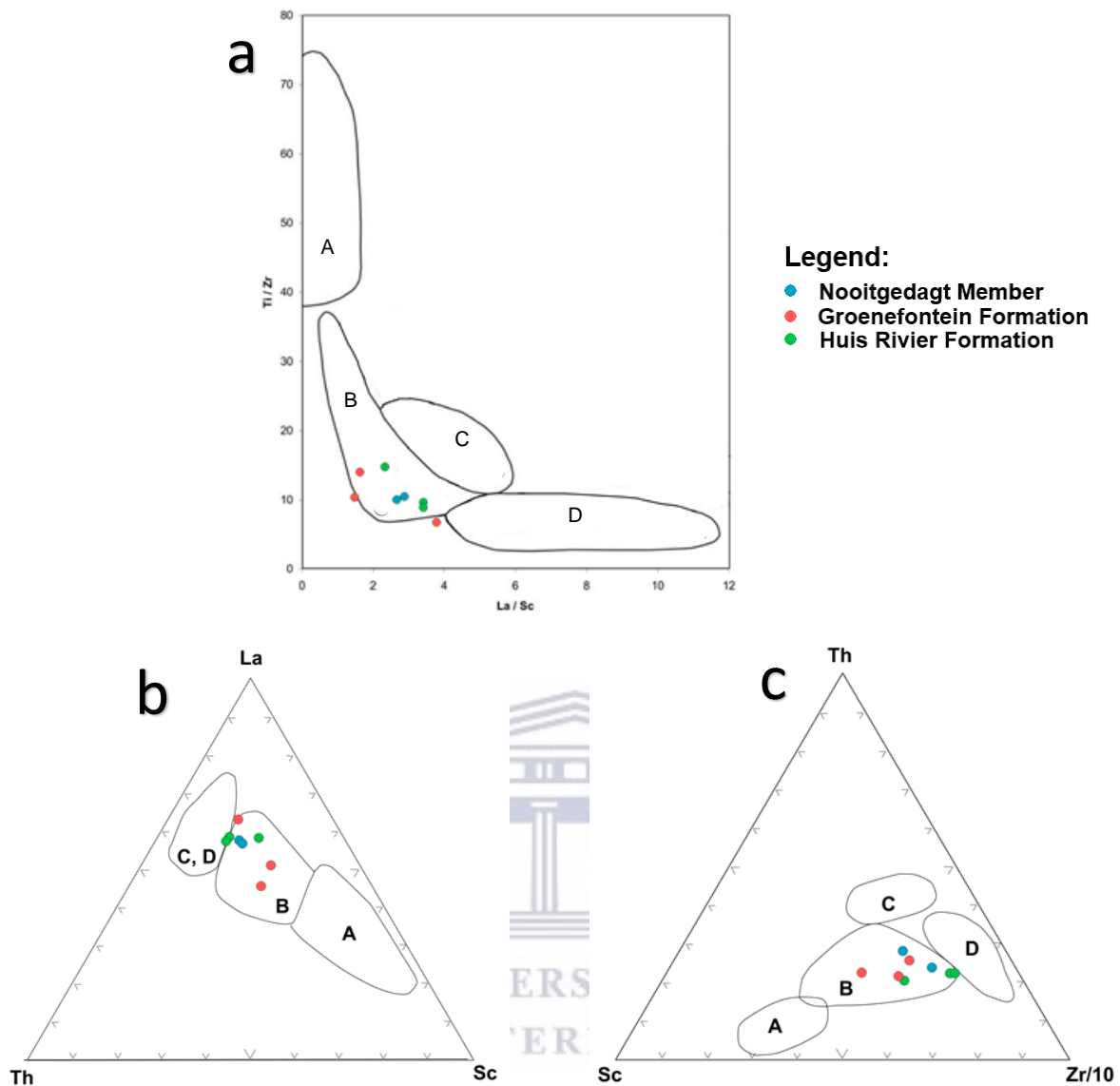
Figure 4-15: Trace element tectonic discriminant diagrams. a – Ti/Zr vs La/Sc; b – Th-La-Sc; c – Sc-Th-Zr/10, after Bhatia and Crook (1986). A = Oceanic Island Arc; B = Continental Island Arc; C = Active Continental Margin; D = Passive Margin.
