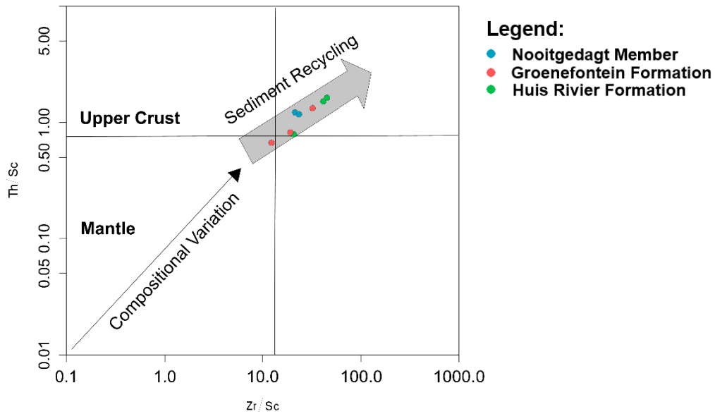
Figure 4-14: Th/Sc vs Zr/Sc ratios of samples of the Cango Caves Group. After McLennan et al. (1990).
