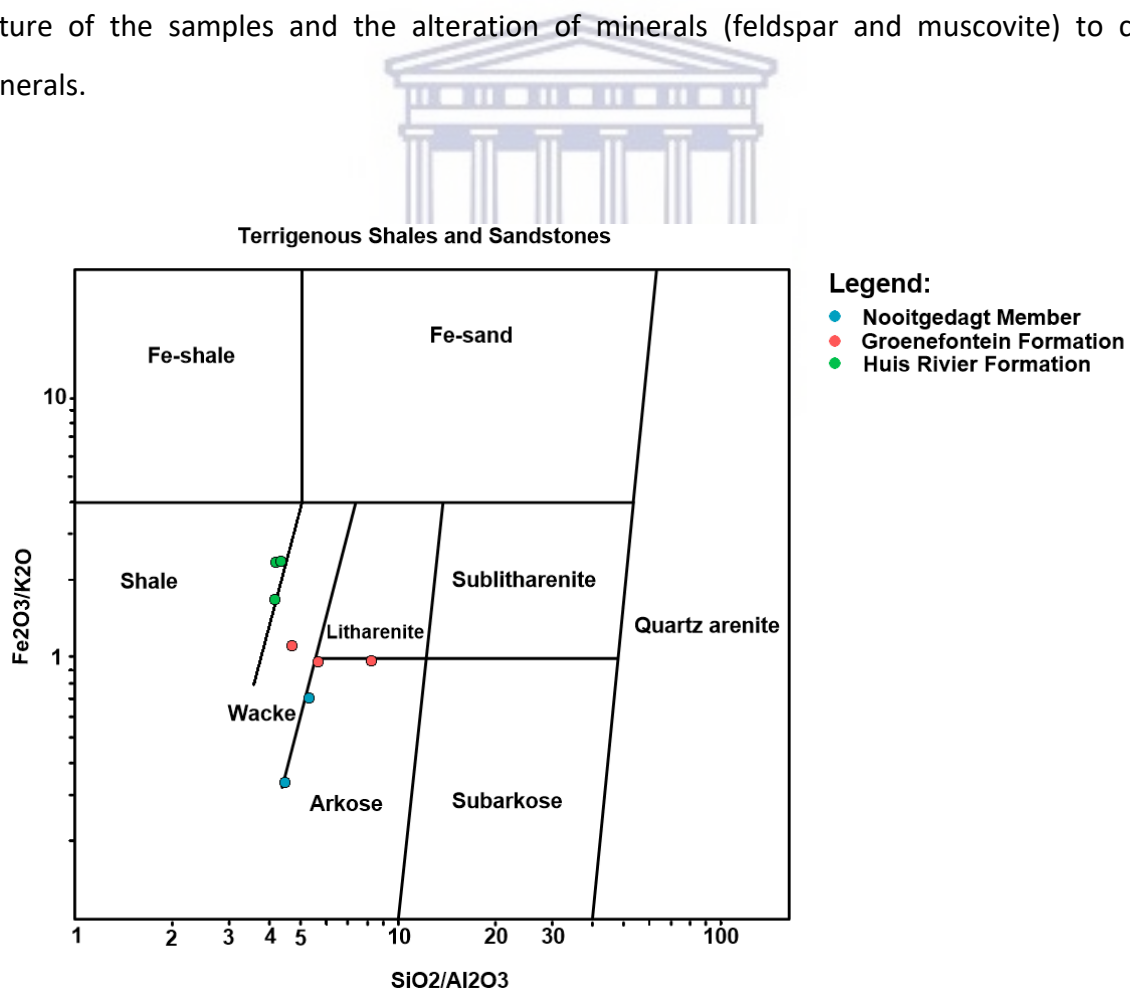
Figure 4-7: \log (\text{SiO}_2/\text{Al}_2\text{O}_3) versus \log (\text{Fe}_2\text{O}_3/\text{K}_2\text{O}) discrimination diagram of Herron (1988) showing the sedimentary rock classification of the Congo Caves Group samples.
