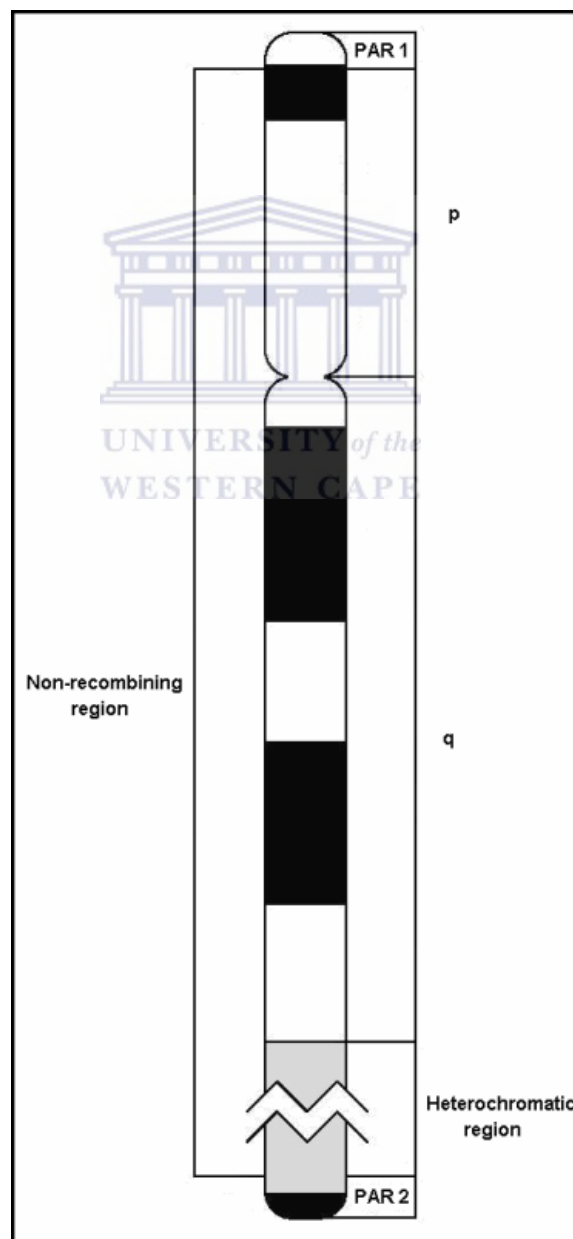
Figure 1.1. Simplified Y-chromosome structure representing the 3 regions: pseudo- autosomal (PAR1 and PAR2), heterochromatic and the non-recombining (Jobling and Tyler-Smith, 2000).
