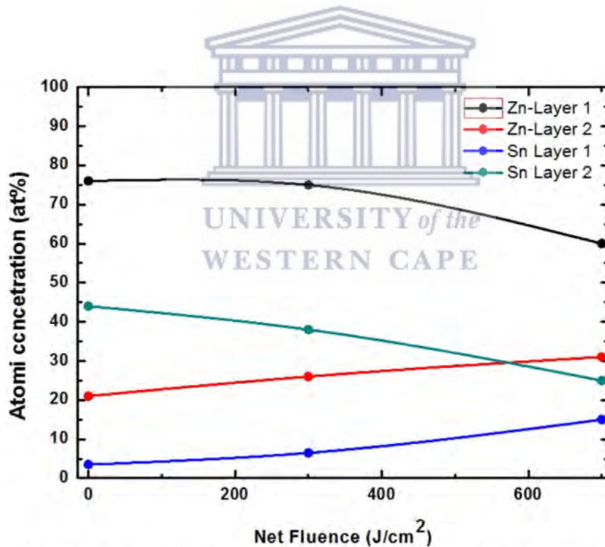
Figure 4.26: Plot of the diffusion depth profiling from the RBS raw data simulations.
