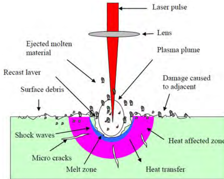
Figure 2.6: Schematic diagram of the interaction of laser with matter [2.32].
