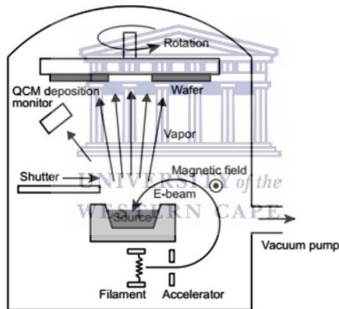
Figure 1.4: Schematic diagram of electron beam evaporation system [1.11].
