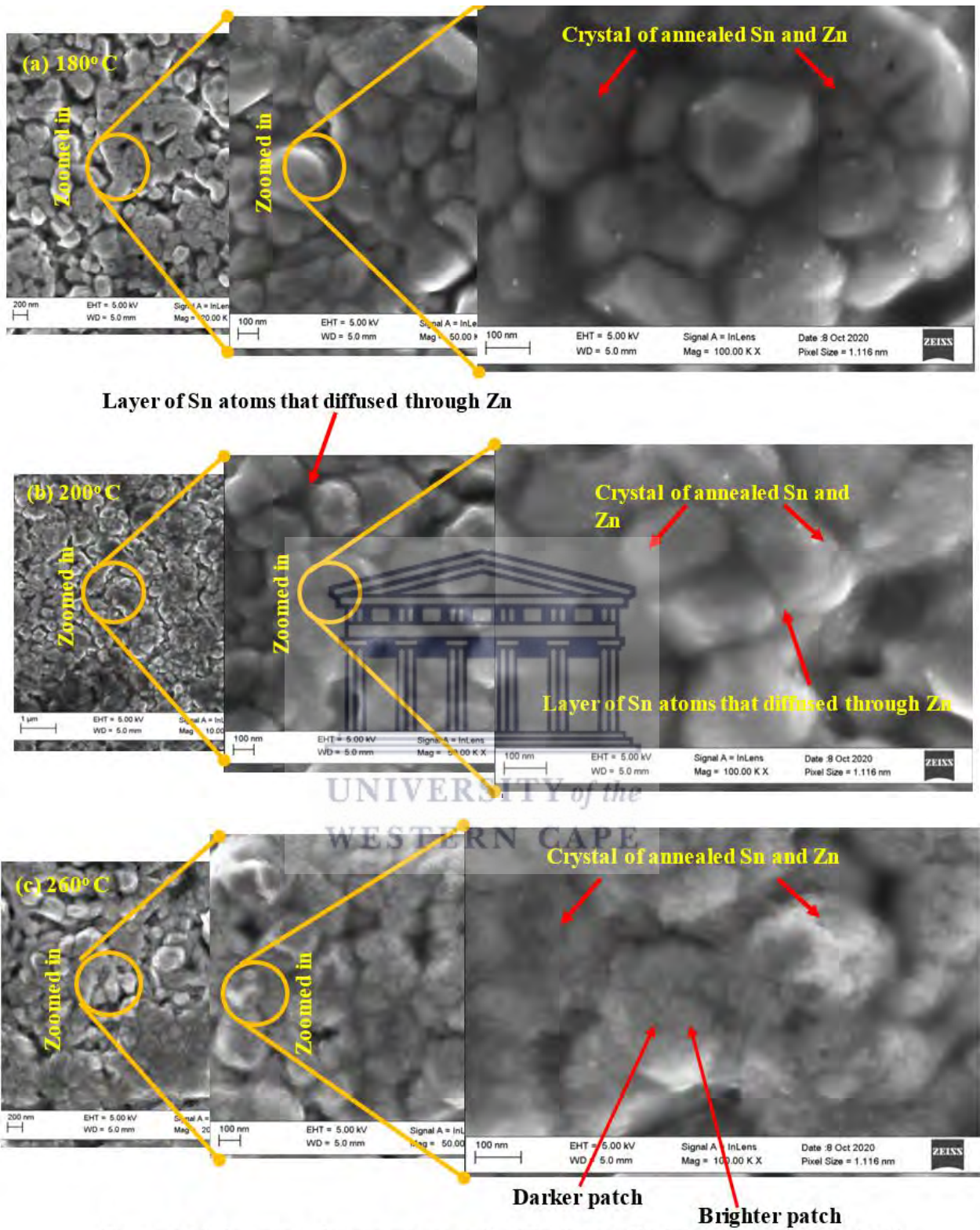
Figure 4.19: Scanning electron micrograph of Zn-Sn metallic bilayer annealed at a) 180 °C, b) 200 °C and c) 260 °C.
