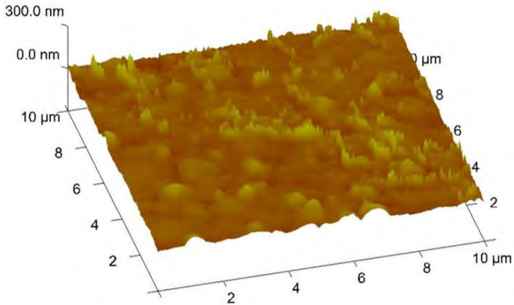
Figure 4.2: AFM micrograph showing surface morphology of pristine Sn on a glass substrate.
