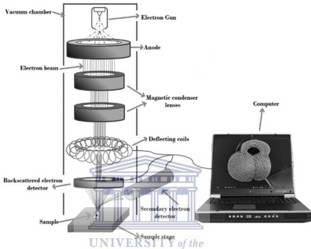
Figure 3.20: Schematic diagram showing the components of scanning electron microscopy [3.30].
