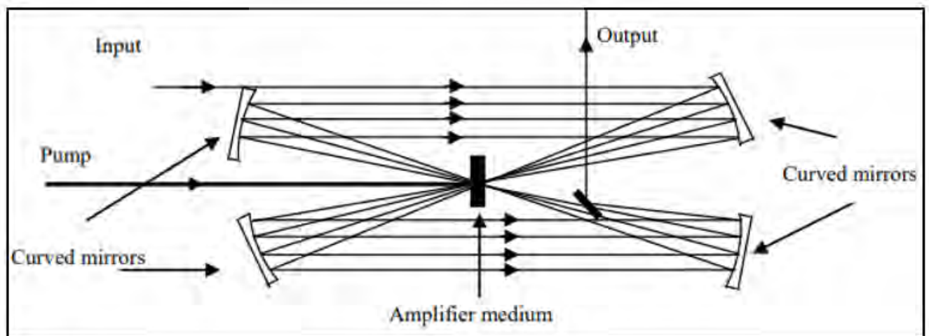
Figure 3.16: Schematic diagram of a multipass amplifier [3.25].
