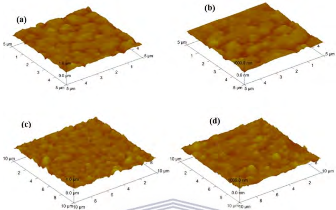
Figure 4.21: AFM micrograph showing surface morphology of Zn-Sn bilayer: a) Pristine, b) bilayer annealed at 180 °C, c) bilayer annealed at 200 °C and d) bilayer annealed at 260 °C.
