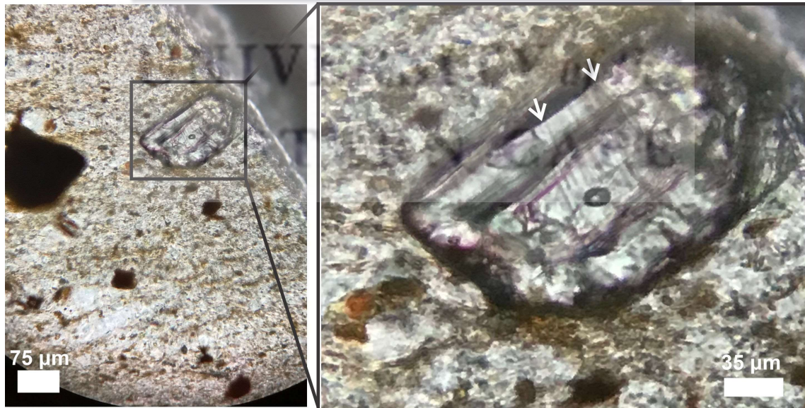
Figure 27: A transmitted light, plane-polarized light photomicrograph of a possible shocked zircon grain with one set of possible planar features that crosscut the growth zoning. The shocked zircon is in thin section TNS1.
