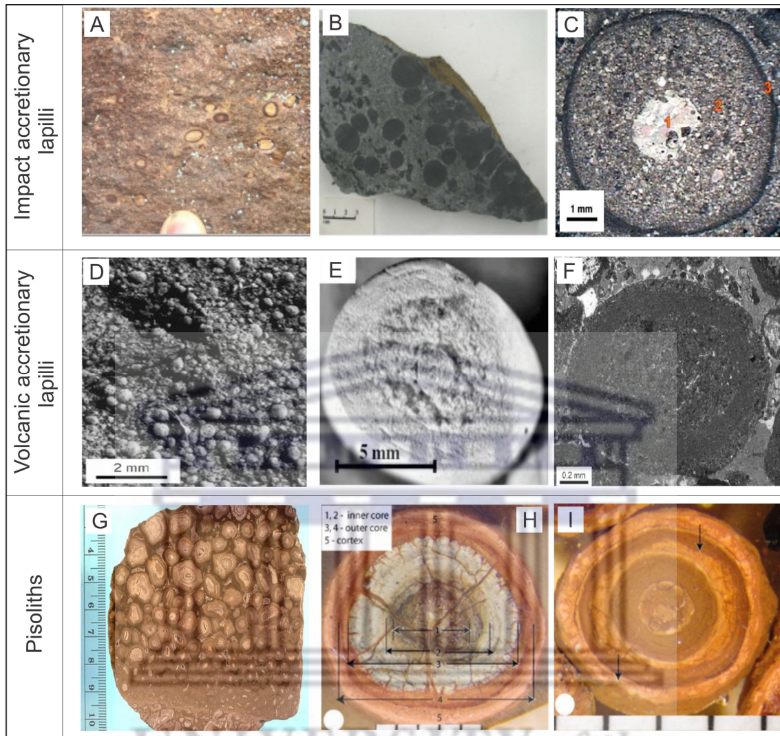
Figure 53: Impact accretionary lapilli, volcanic accretionary lapilli, and pisolites/pisoliths. (A) Impact accretionary lapilli from Stac Fada Member in Scotland with a concentric structure consisting of nuclei, mantles and crusts (Osinski et al. 2021). (B) A sample with impact accretionary lapilli from Hillcrest Part from the Sudbury impact ejecta (Huber & Koeberl, 2017). (C) A photomicrograph of a carbonaceous impact accretionary lapillus, where (1) indicates the nucleus, (2) a graded mantle and (3) the crust (Morgan, 2006). (D) A volcanic accretionary lapilli-rich layer in the Tumbiana Formation of the Hamersley Basin in Australia (Glass & Simonson, 2013). (E) An ultrafine accretionary lapillus with a nucleus, mantle and crust from the Oruanui ignimbrite proximal facies in New Zealand (Kósik et al. 2019). (F) A volcanic accretionary lapillus showing a concentric structure with a nucleus, mantle and crust from the Tumbiana Formation in the Hamersley Basin (Glass & Simonson, 2013). (G) A pisolitic dolomite polished slab in New Mexico from Yates Formation in the USA (Scholle, 1999). Note the reverse grading of grains and the fitting fabric, where grains have interlocking boundaries caused by compromised outer growth. (H & I) Pisoliths from Jacaranda pit in Australia. (H) A complex pisolith from Jacaranda with a cortex surrounding an inner core and outer core. (I) Pisoliths from Jacaranda with scour and fill (indicated by the arrow). Figures (H & I) were obtained from Taylor (2008).
