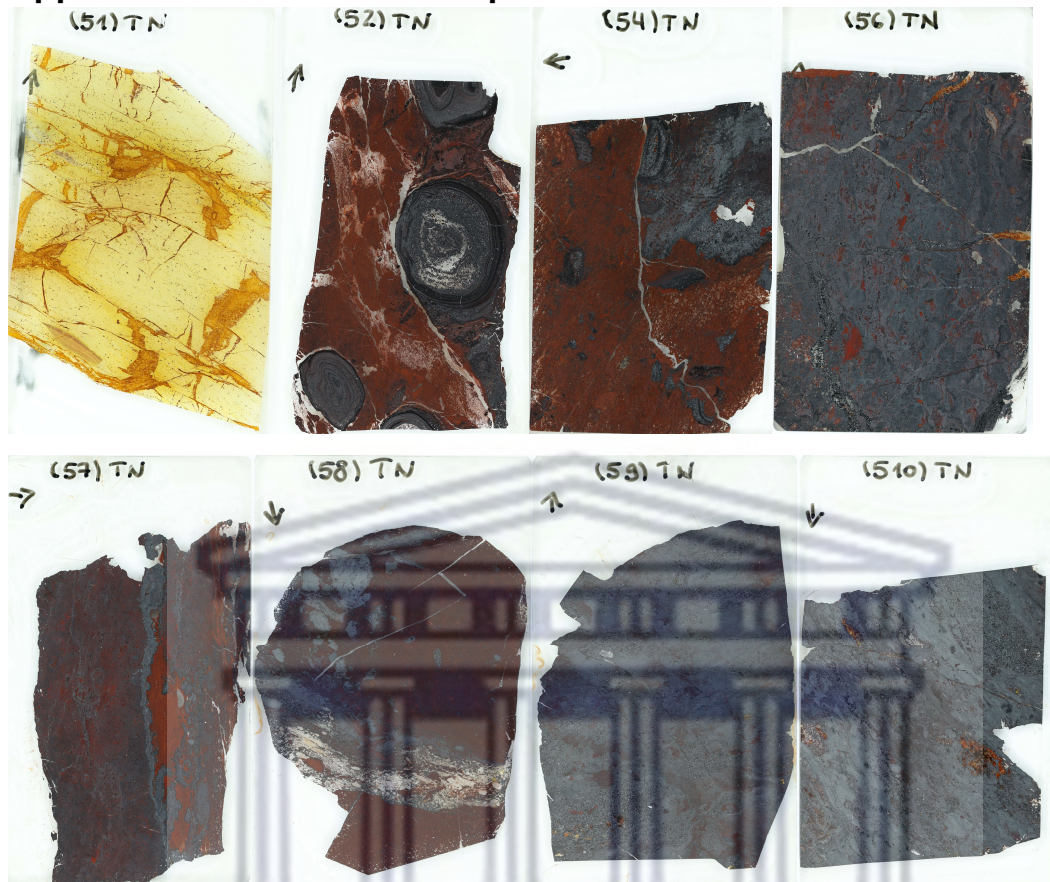
B.2.1: As indicated on the thin sections, these are thin section photos of TNS1, TNS2, TNS4, TNS6, TNS7, TNS8, TNS9 and TNS10.
