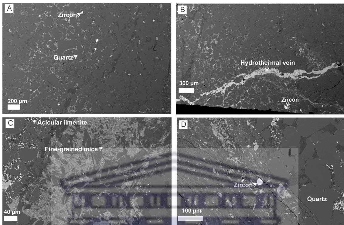
Figure 29: (A-D) SEM Photomicrographs of the sample TNS18; the white arrows show the minerals. Note the angular grains of quartz and zircon occurring in a matrix comprised of acicular fine-grained mica and acicular ilmenite. Also, note the hydrothermal vein rich in Fe-oxide in (B).
