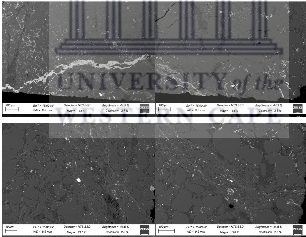
A.3.6: BSE images of matrix of TNS18.
