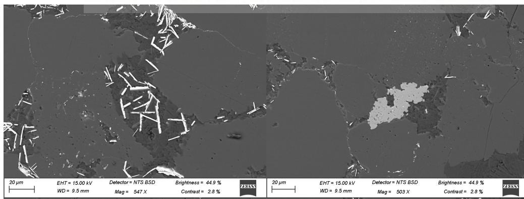
A.3.4: BSE images of quartz and zircon grains in a fine-grained matrix consisting of acicular ilmenite in TNS18.
