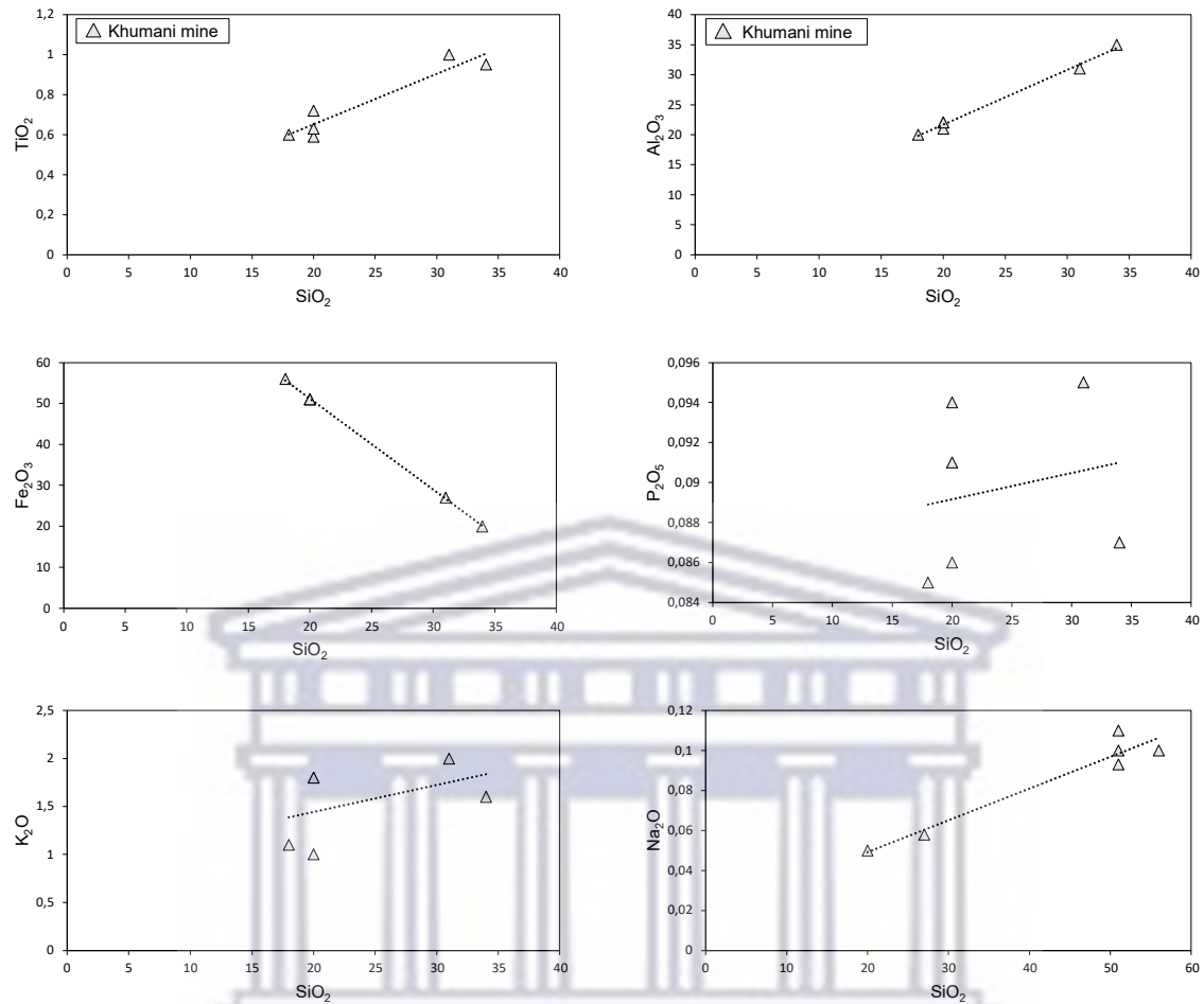
Figure 17: \text{SiO}_2 vs \text{TiO}_2 , \text{K}_2\text{O} , \text{Na}_2\text{O} , \text{Al}_2\text{O}_3 , \text{P}_2\text{O}_5 and \text{Fe}_2\text{O}_3 Harker diagrams for the samples from Khumani Mine. The dotted lines represent linear regression lines/correlations for the Harker diagrams. Note the positive correlations between \text{SiO}_2 and \text{TiO}_2 , \text{K}_2\text{O} , \text{Na}_2\text{O} , \text{Al}_2\text{O}_3 , and \text{P}_2\text{O}_5 and a negative correlation between \text{SiO}_2 and \text{Fe}_2\text{O}_3 for the samples.
