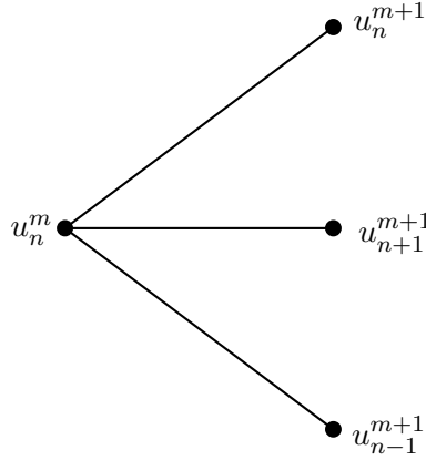
Figure 5.3: Implicit Finite difference discretisation
