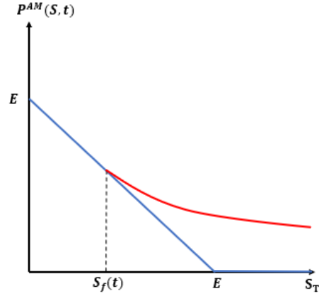
Figure 3.8: \frac{\partial P^{AM}}{\partial S_f(t)} > -1
