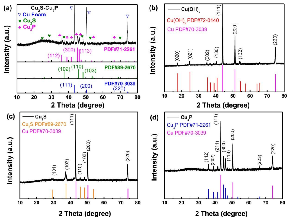
Figure 4.1 XRD curves of the samples with a scan rate of 10^\circ \text{ min}^{-1} . (a) \text{Cu}_2\text{S-Cu}_3\text{P} NW arrays. (b) \text{Cu(OH)}_2 NW arrays, (c) \text{Cu}_2\text{S} NW arrays, (d) \text{Cu}_3\text{P} NW arrays.
