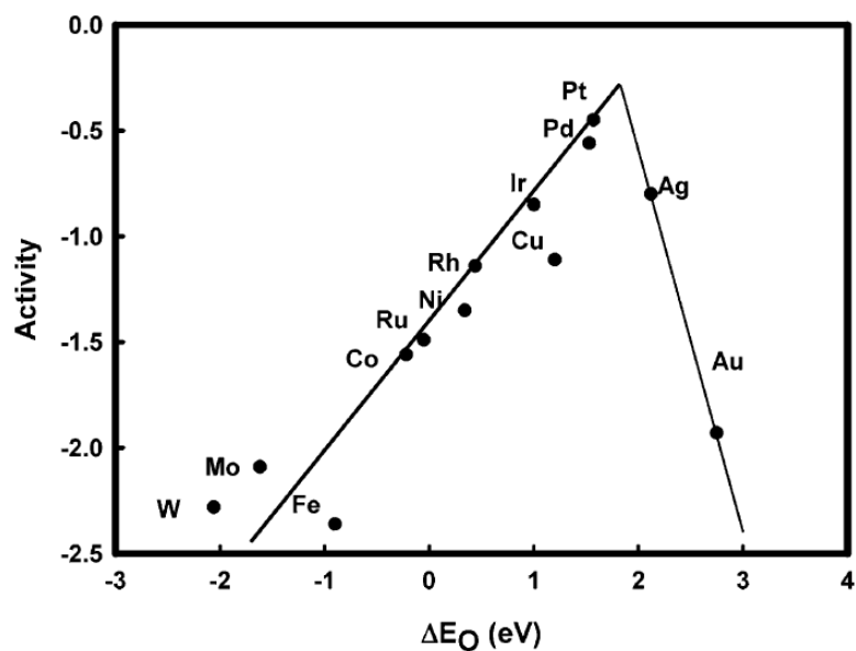
Figure 1.4 Trends in oxygen reduction activity plotted as a function of the oxygen binding energy.[27]
