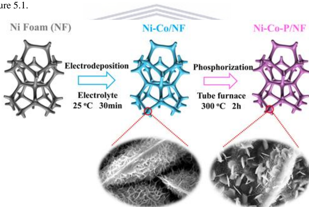
Figure 5.1 Schematic illustration for the synthesis of Ni-Co-P/NF.
