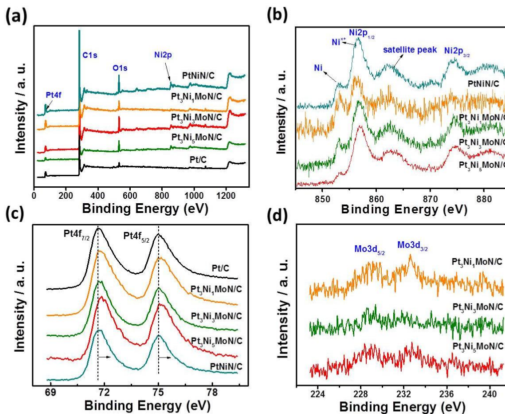
Figure 3.7 (a) XPS spectra of the investigated materials: (b) Ni2p, (c) Pt4f, and (d) Mo3d.
