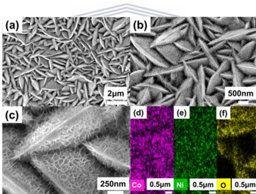
Figure 5.7 SEM (a–c) and EDS (d–f) images of Ni-Co/NF precursor.
