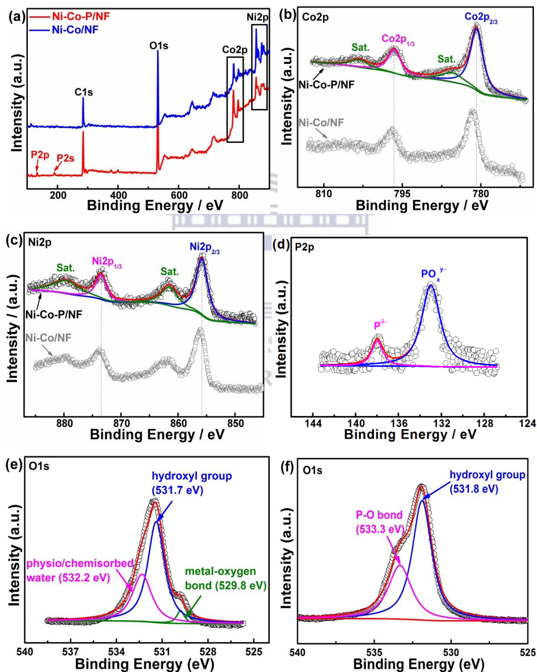
Figure 5.6 (a) XPS summary of Ni-Co-P/NF and Ni-Co/NF, (b) Co2p, (c) Ni2p, (d) P2p and O1s of (e) Ni-Co/NF and (f) Ni-Co-P/NF.
