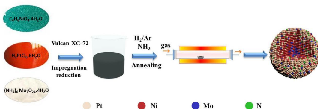
Figure 3.1 Schematic diagram for the synthesis of PtNiMo alloy electrocatalysts.
