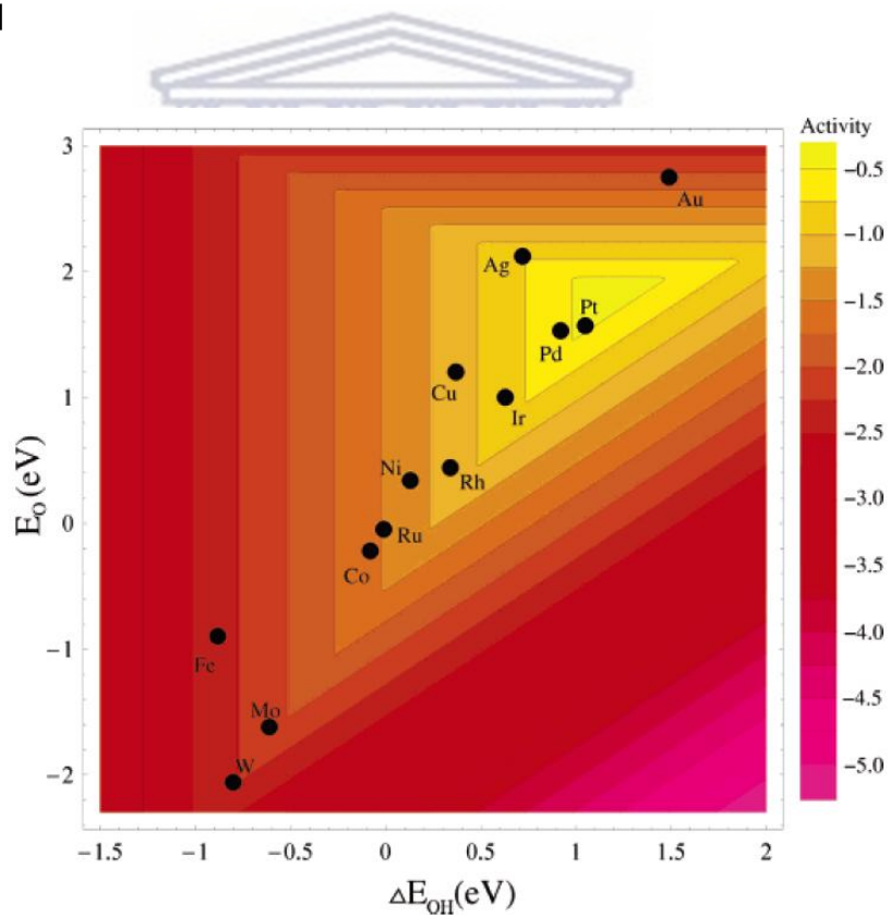
Figure 1.5 Trends in oxygen reduction activity plotted as a function of both the O and the OH binding energy.[27]
