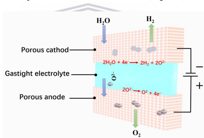
Figure 1.10 Principle of solid oxide water electrolyzer.
