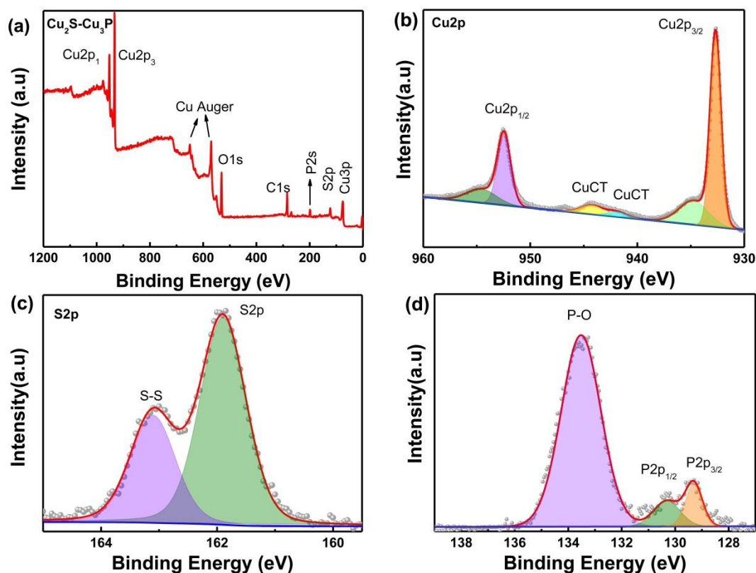
Figure 4.3 (a) XPS summary of \text{Cu}_2\text{S-Cu}_3\text{P} NW arrays, the corresponding (b) \text{Cu}2p , (c) \text{S}2p and (d) \text{P}2p .
