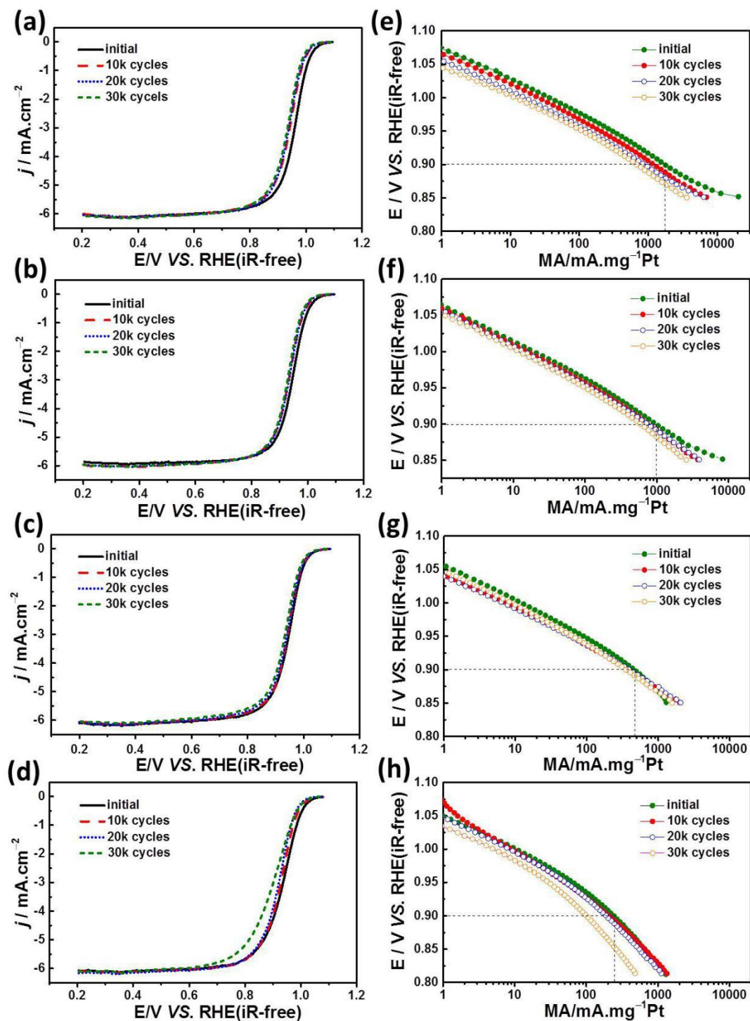
Figure 3.11 (a-d) ORR polarization curves of \text{Pt}_3\text{Ni}_5\text{MoN}/\text{C} , \text{Pt}_3\text{Ni}_3\text{MoN}/\text{C} , \text{Pt}_3\text{NiMoN}/\text{C} and TKK \text{Pt}/\text{C} in \text{O}_2 -saturated 0.1 \text{ mol L}^{-1} \text{ HClO}_4 aqueous solutions before and after ADT, 25^\circ\text{C} , scan rate 5 \text{ mV s}^{-1} , rotating rate 1,600 \text{ rpm} . (e-h) MAs for \text{Pt}_3\text{Ni}_5\text{MoN}/\text{C} , \text{Pt}_3\text{Ni}_3\text{MoN}/\text{C} , \text{Pt}_3\text{NiMoN}/\text{C} compared with \text{Pt}/\text{C} before and after 30k cycles.
