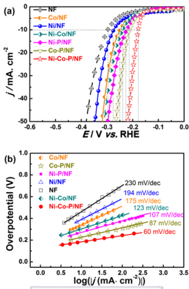
Figure 5.17 (a) The normalized HER activities (current density) by their ESCAs; (b) the corresponding Tafel slopes.
