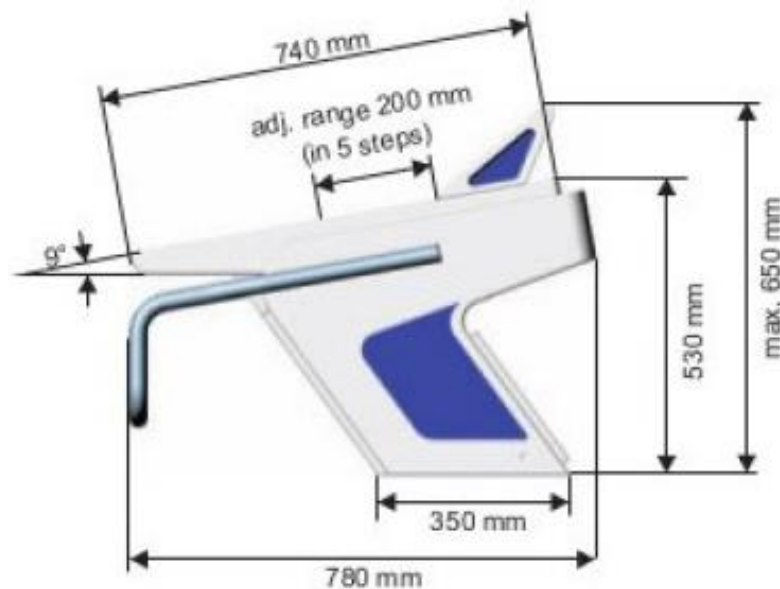
Figure 2. 3: Omega OBS11 Starting Block (HTS Group Ltd, 2000)
