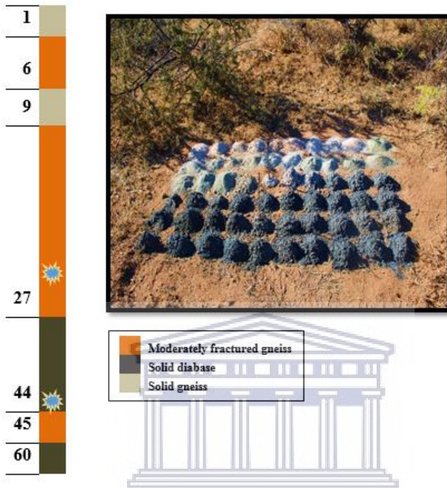
Figure 6.3 Well profile and sample images for borehole HO4-3125
