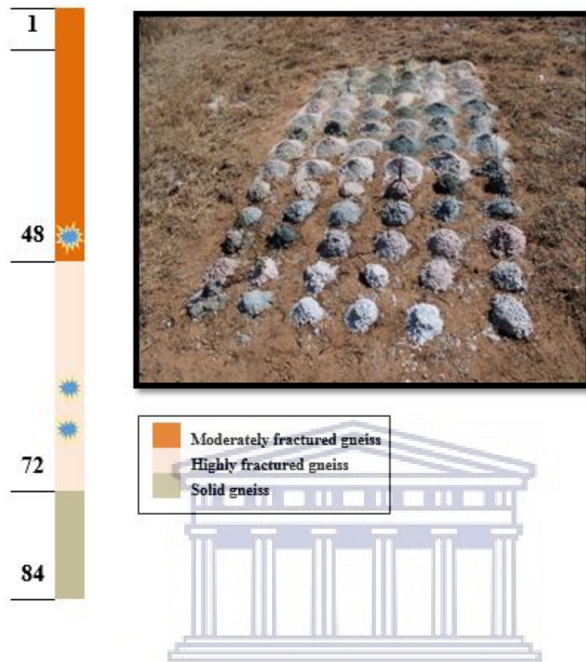
Figure 6.4 Well profile and sample images for borehole HO4-3126
