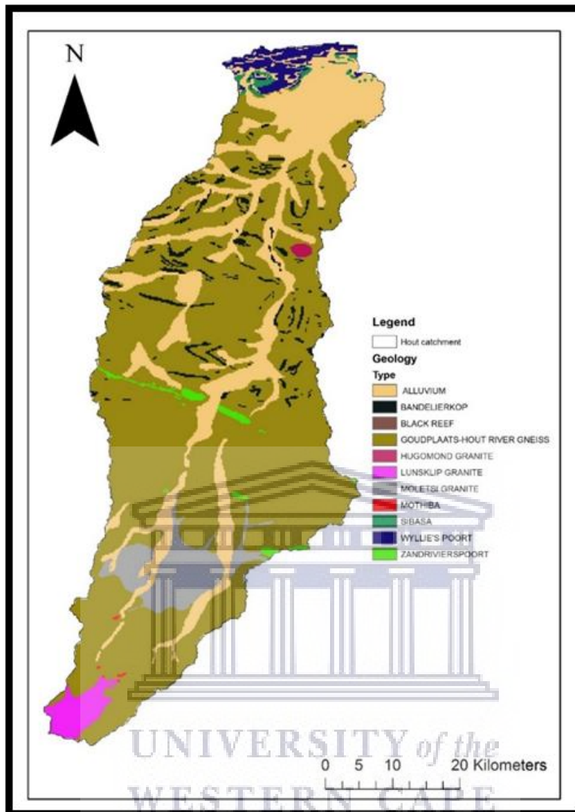
Figure 5.1 Geological map of the study area (based on the geological map of South Africa)
