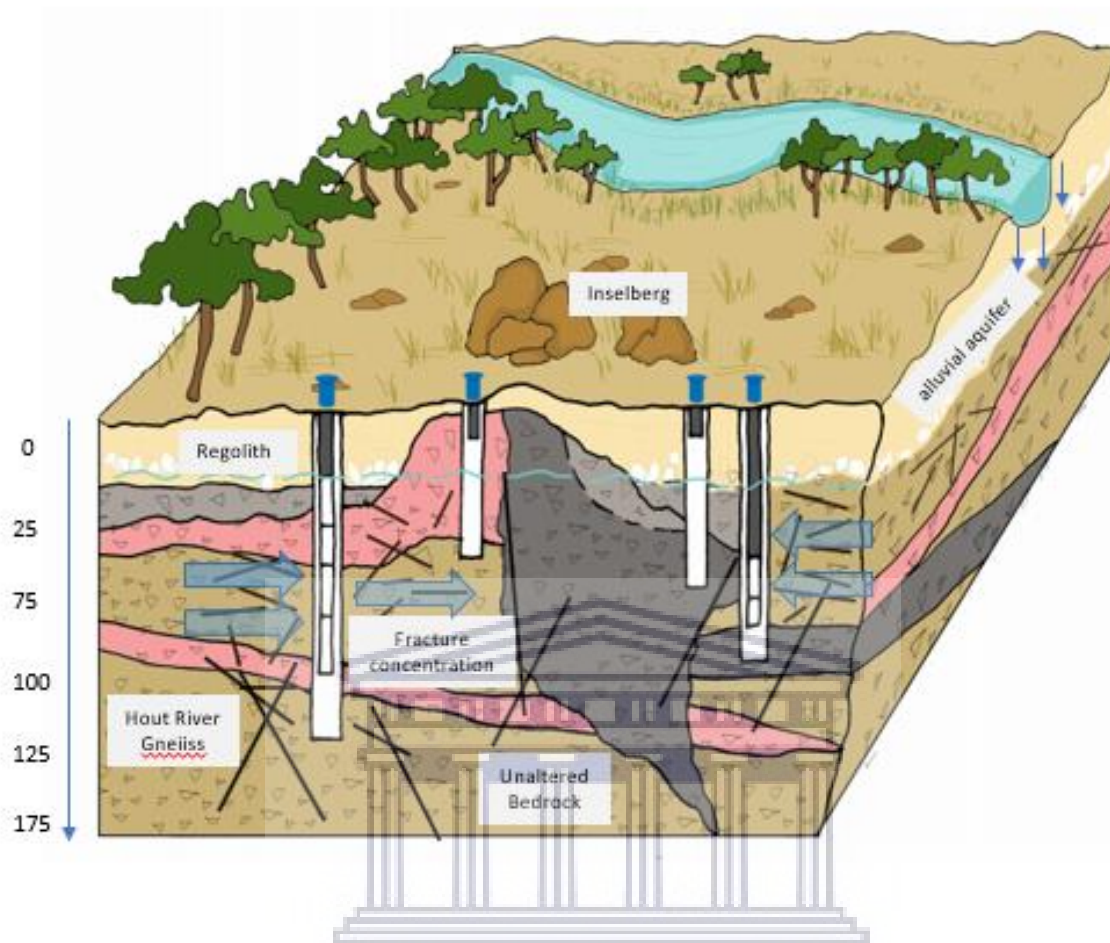
Figure 7.1 Hydrogeological conceptual model of Ga-Mamadila experimental site
