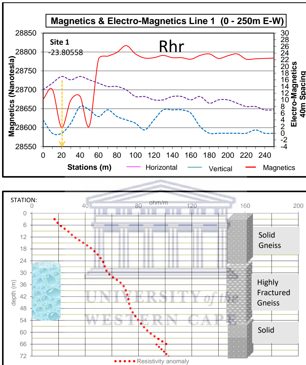
Figure 5.8 a) Variation of magnetic susceptibility, the horizontal and vertical FDEM results along profile line 1 (b) The corresponding vertical electrical resistivity section together with the inferred depth variation profile from electrical resistivity result.
