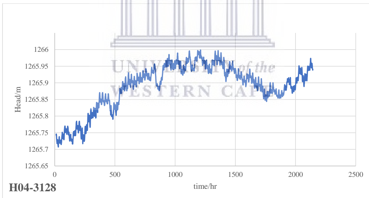
Figure 6.17 (a-d). Time series variation of hydraulic heads with time from 31 October 2019 to 27 January 2020
