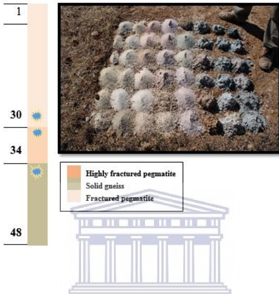
Figure 6.6 well profile and sample images for borehole HO4-3128
