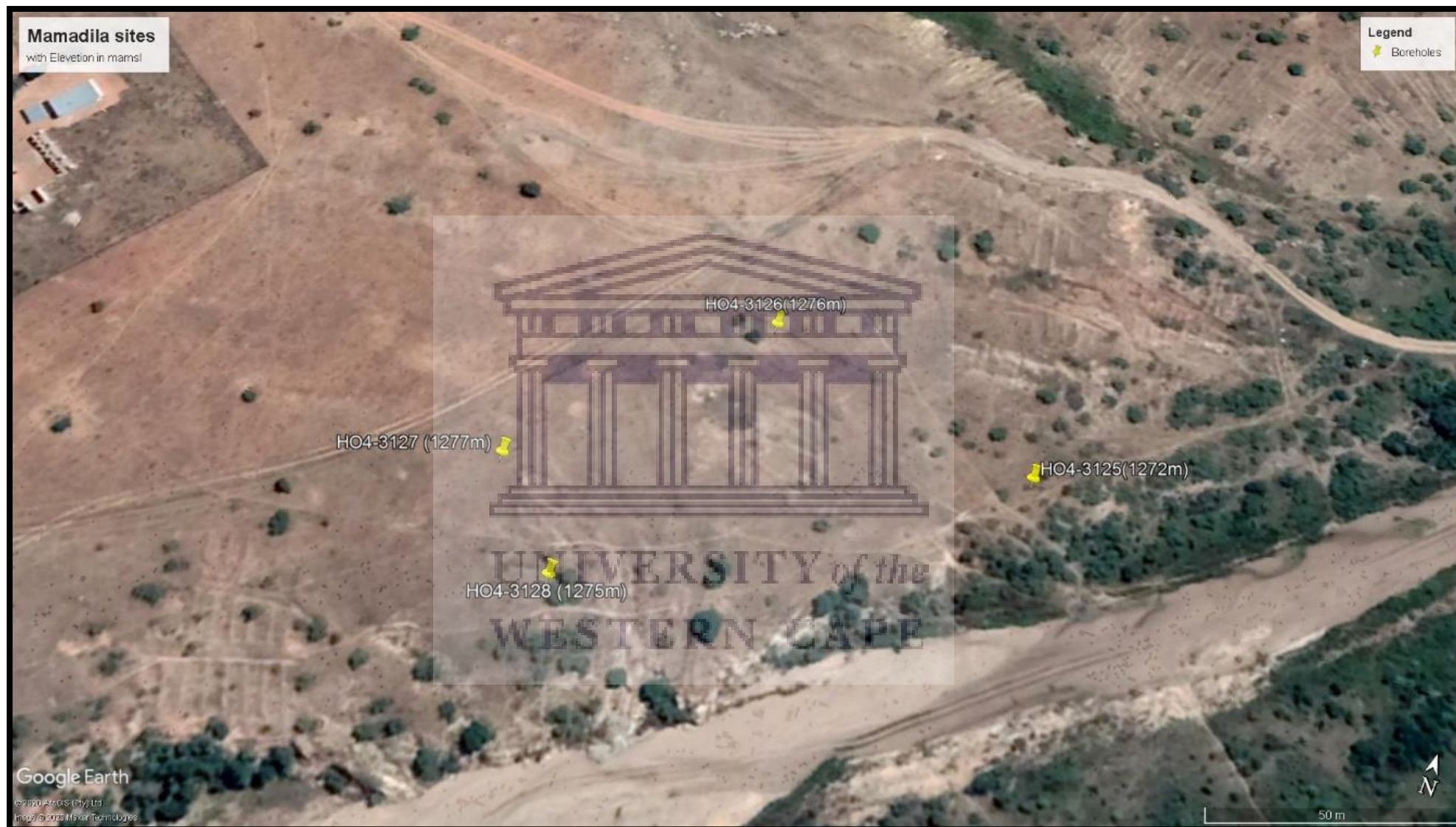
Figure 4.6 Borehole sites within the Ga-Mamadila community
