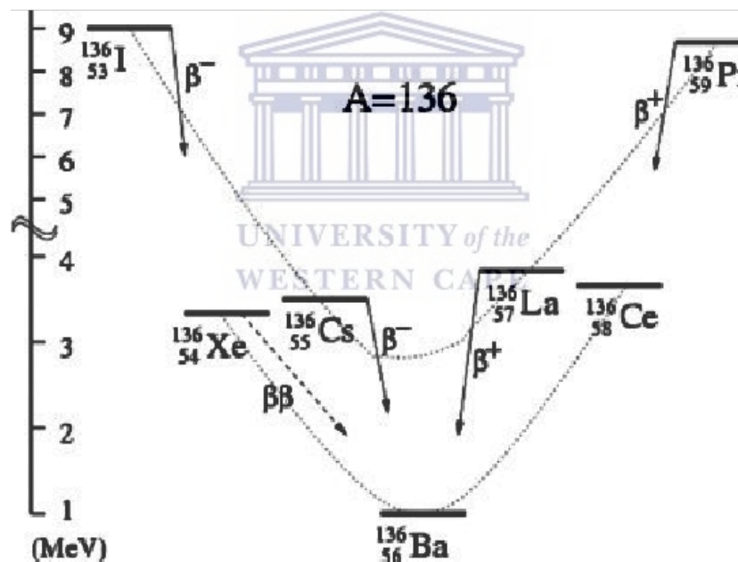
Figure 1.5: Mass parabola for A = 136 isobars. Although ^{136}\text{Xe} cannot \beta decay to ^{136}\text{Cs} , \beta\beta decays to ^{136}\text{Ba} are allowed. Figure taken from Ref [17].
