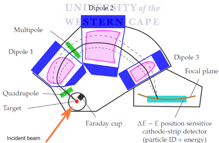
Figure 3.4: The Q3D magnetic spectrograph, illustrating the trajectory of a light charged ejectile to the focal plane.
