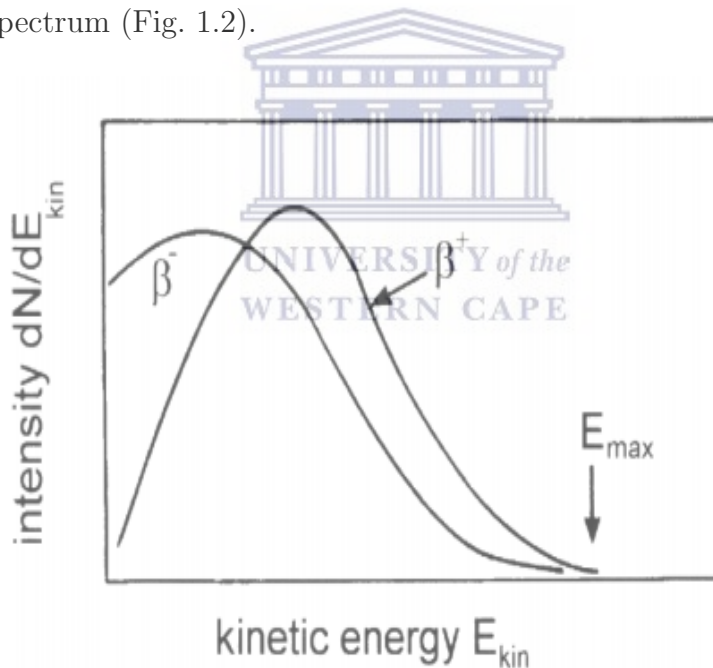
Figure 1.2: Energy distribution of electrons and positrons observed during beta decays. Figure taken from Ref. [4].
