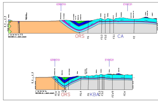
FIGURE 4.14.A.4 - HYDROGEOLOGICAL
