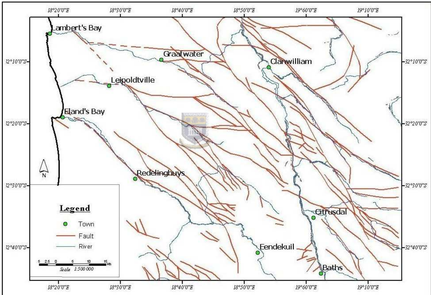
Figure 4.4 Drainage and fault orientation.
