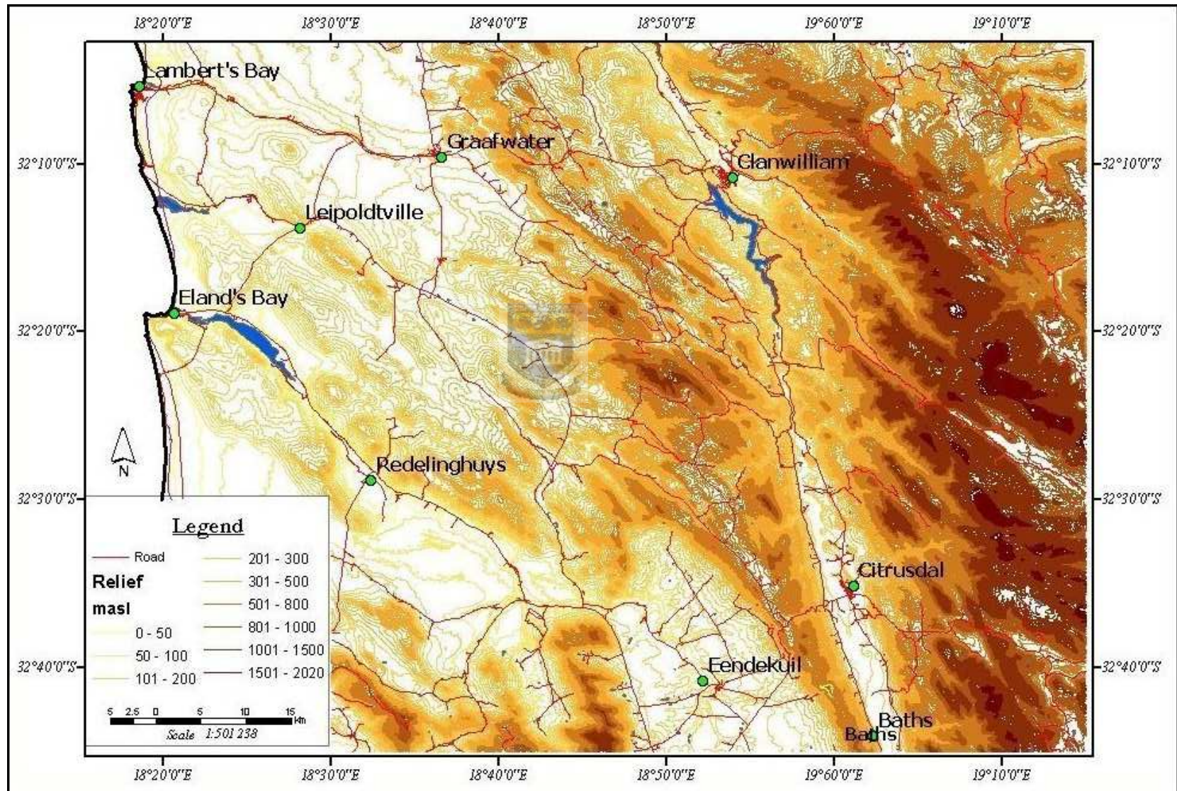
Figure 4.5 Topographic map showing the relief of the aerea.
