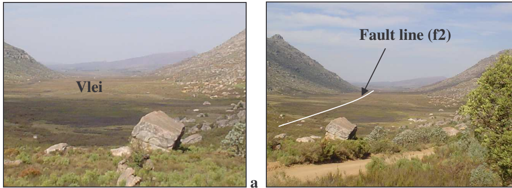
Figure 5.17a&b Mountain- top vleis in the Cederberg Pass.
