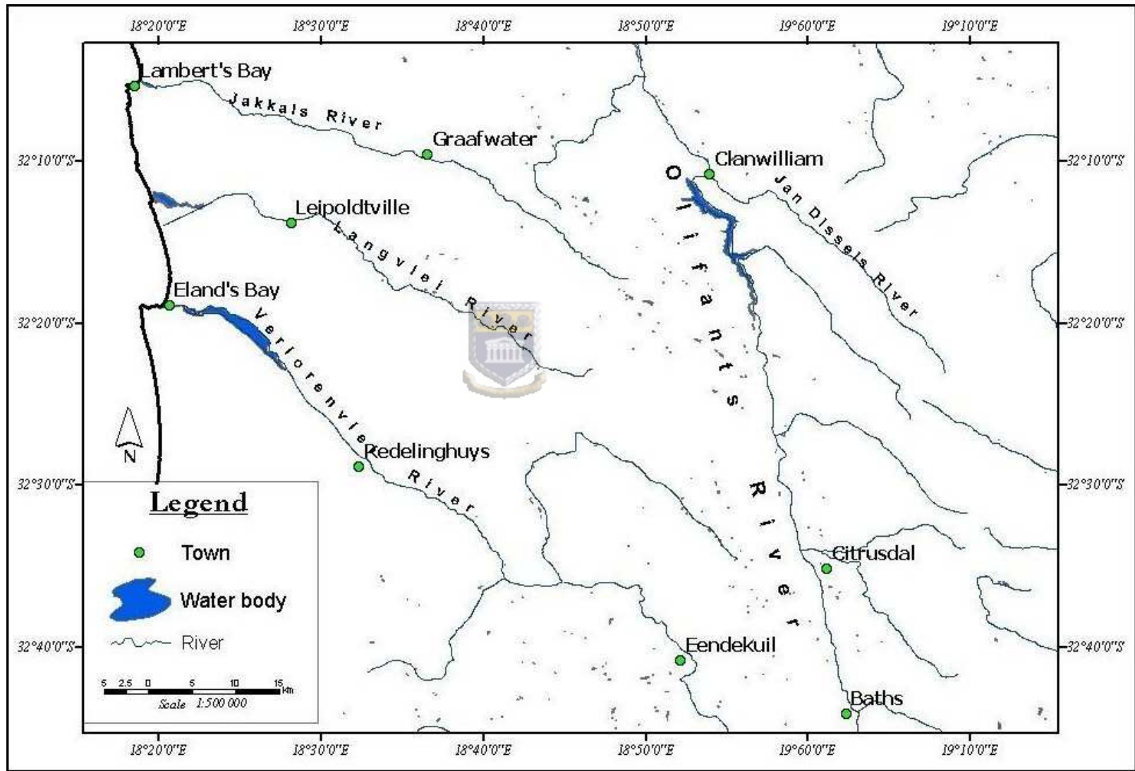
Figure 4.2 Main drainage features of area.
