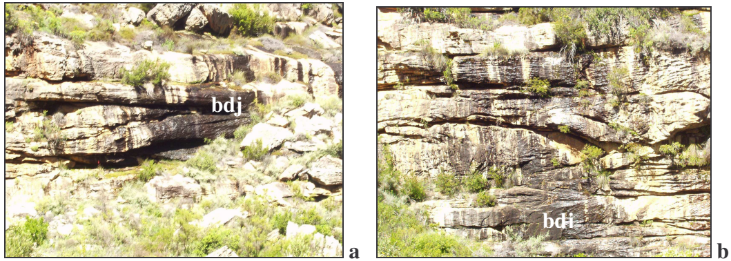
Figure 5.10 a & b Water seeping out of bedding joints in Nardouw Subgroup, Pakhuisberg Pass.
