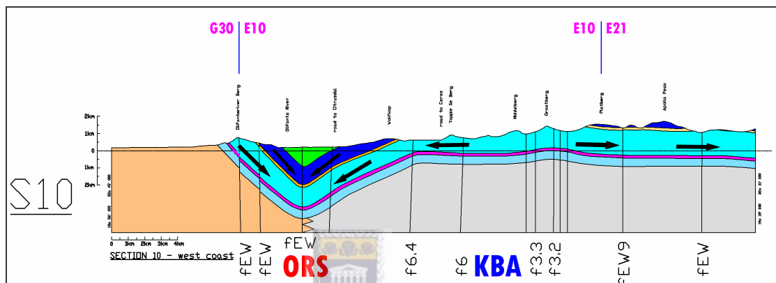
Figure 4.16 j Cross section 10 showing flow direction.
