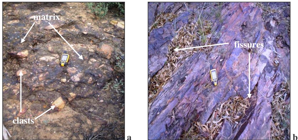
Figure 5.3 a & b Fault breccia and shear in fault zone, Clanwilliam.
