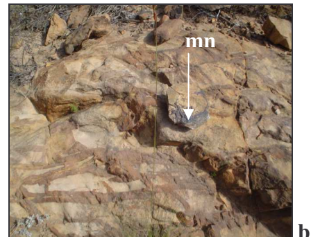
Figure 5.1b Iron & manganese staining
