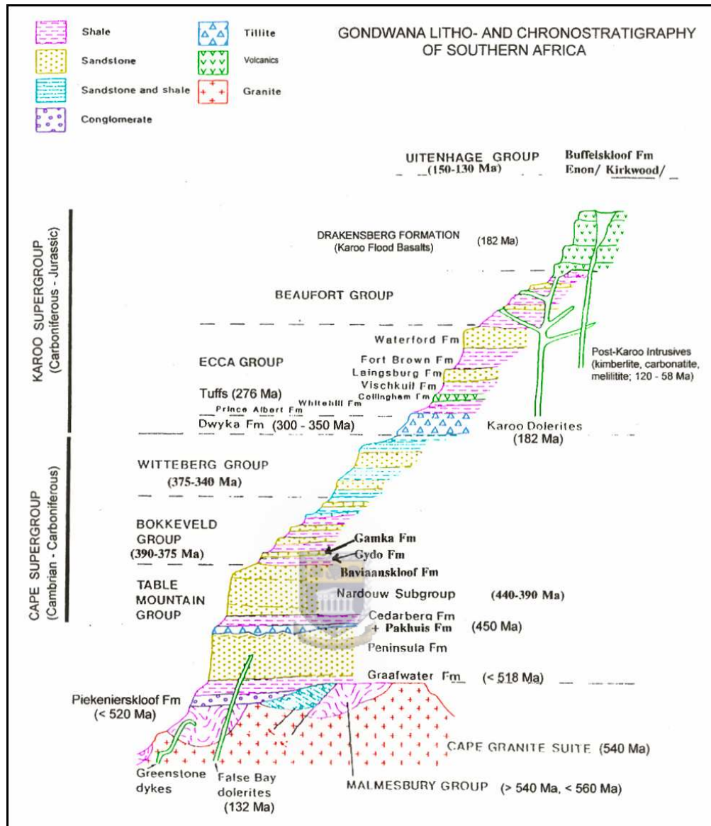
Figure 4.7 Cape and Karoo Supergroup sequence (modified from Reid et al, 1998)
