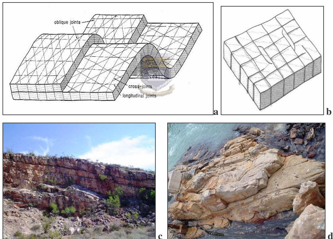
Figure 4 12 a, b, c, d Joint sets in fractured rocks (a, b). Examples of joint patterns in folded Nardouw Subgroup, showing strong bedding joints (c) and in Piekensklouf Formation (d) showing bed, long and cross joints. (a and b from Roberts, 1982).
