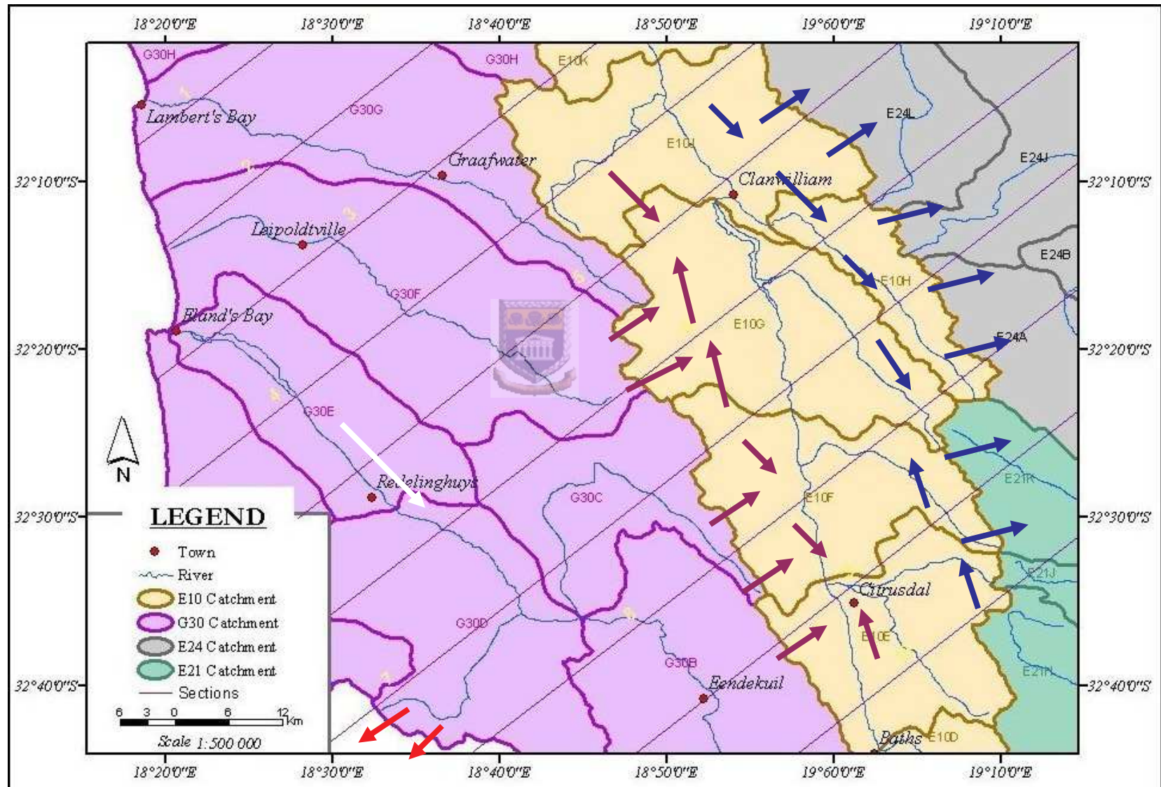
Figure 5.19 Inter catchment flow as indicated on cross sections (arrows show deep flow directions in the lower aquifer)
