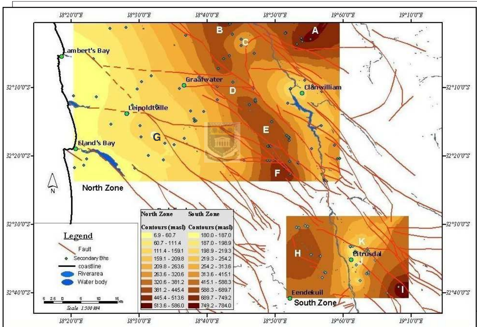
Figure 5.13 Water level contours for the Secondary TMG aquifer (using ordinary Kriging). Arrow lines show flow direction.
