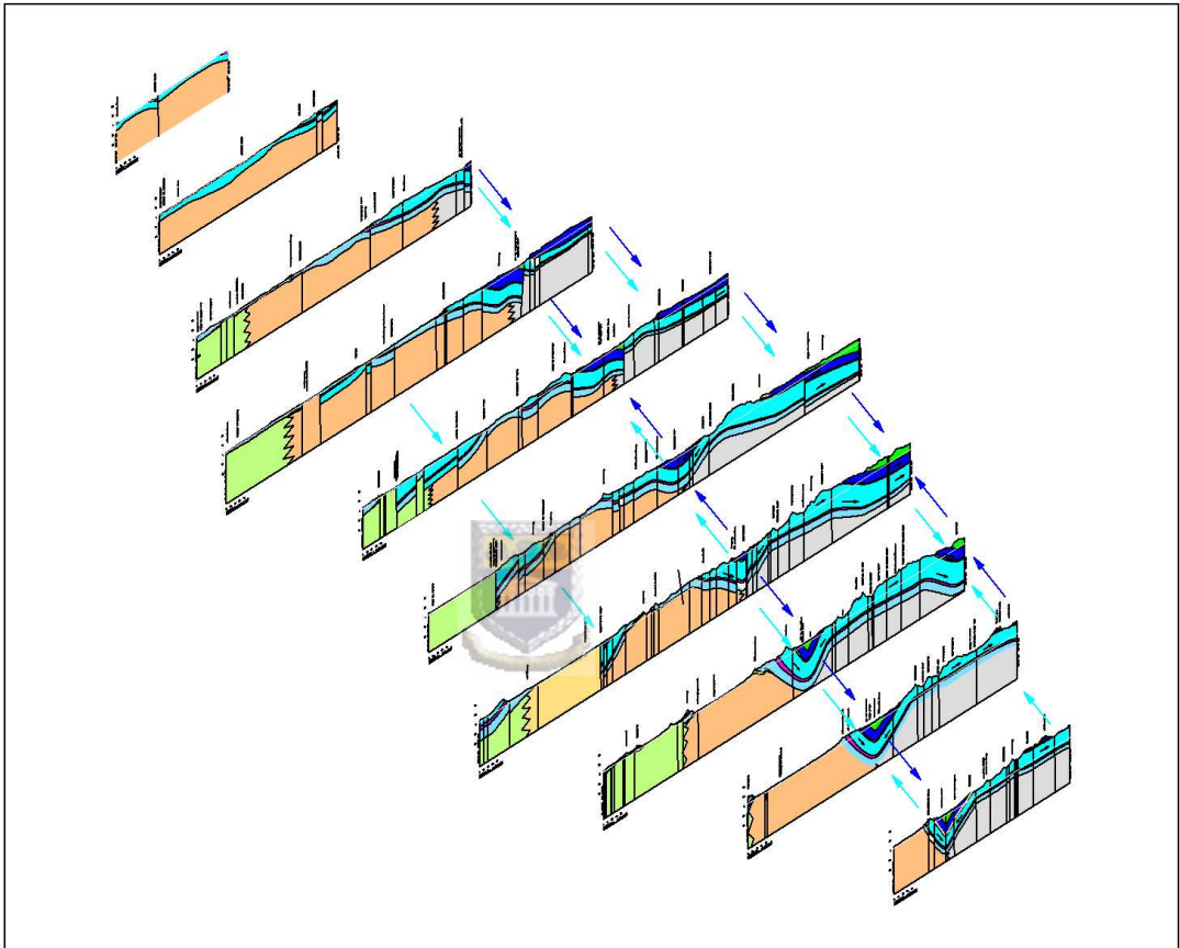
FIGURE 4.15 Isometric flow sections
