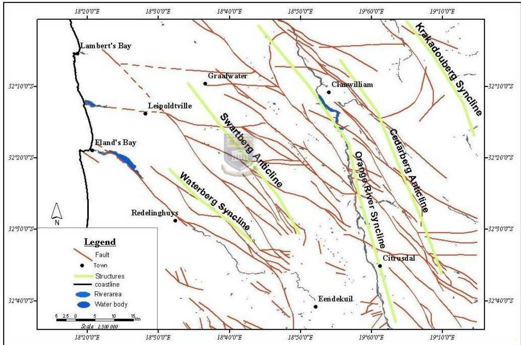
Figure 4.11 Faults and fold structures of the study area.
