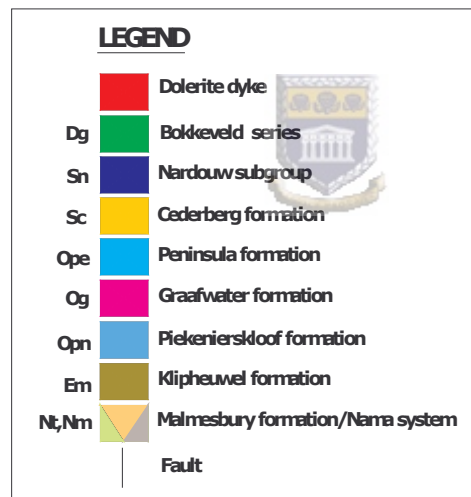
Figure 4.16 Stratigraphic sequence for cross sections below
