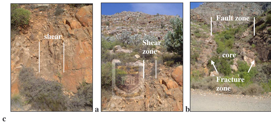
Figure 5.2 a,b & c Two different fault types in the Cederberg Mountains near Algeria.
