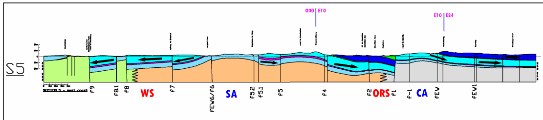
Figure 4.16 e Cross section 5 showing flow direction.
