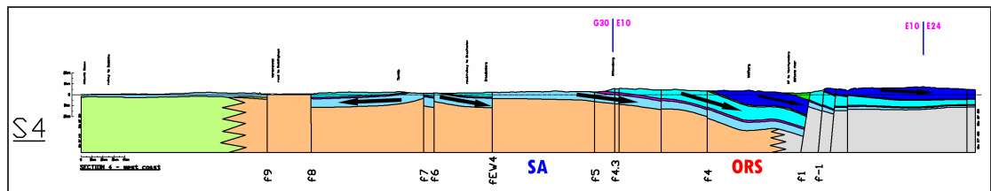
Figure 4.16 d Cross section 4 showing flow direction.
