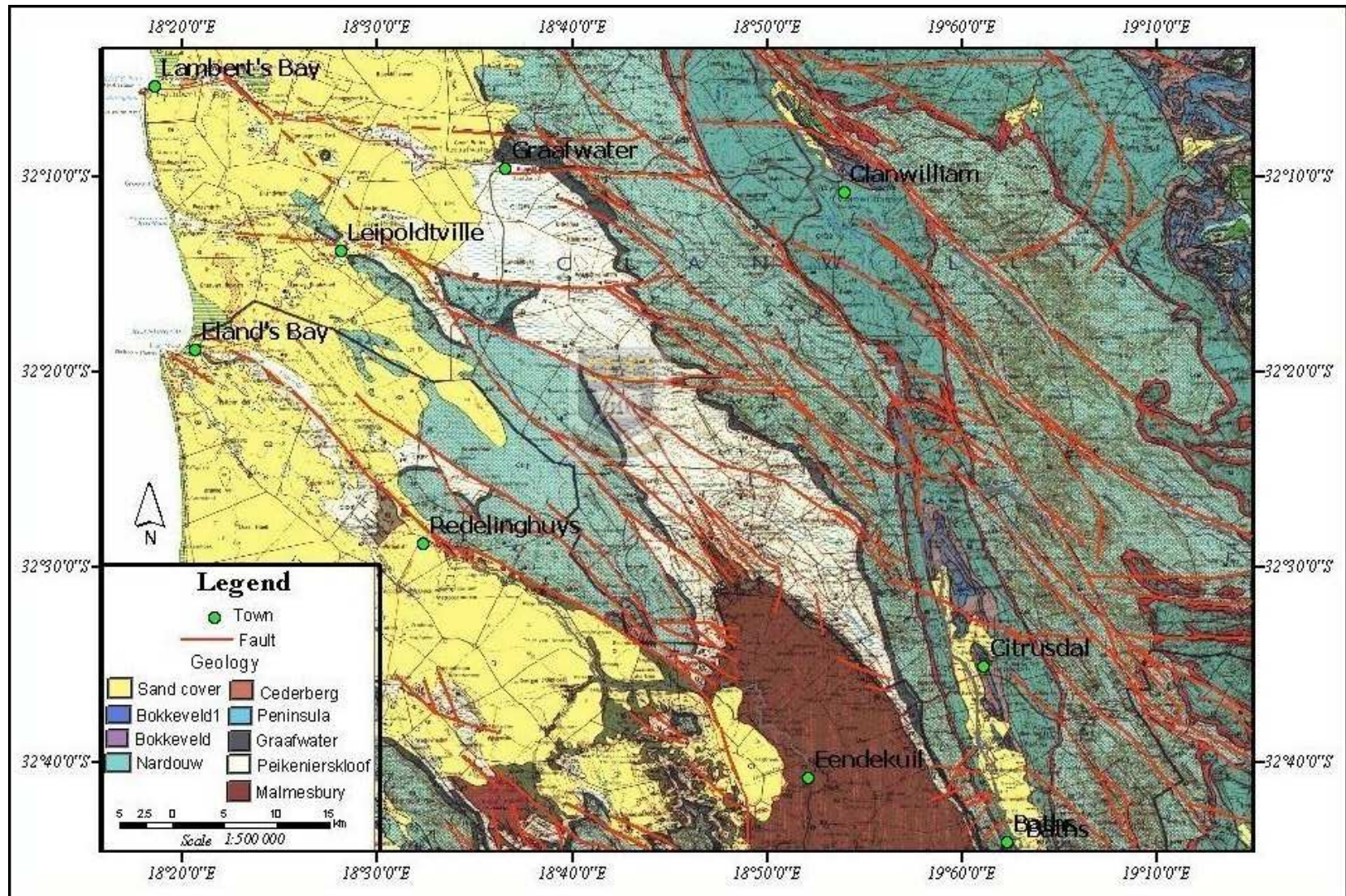
Figure 4.9 Geological map of Clanwilliam showing main faults (based on published 1:250000 map,3218Clanwilliam,1973,Council For Geoscience)
