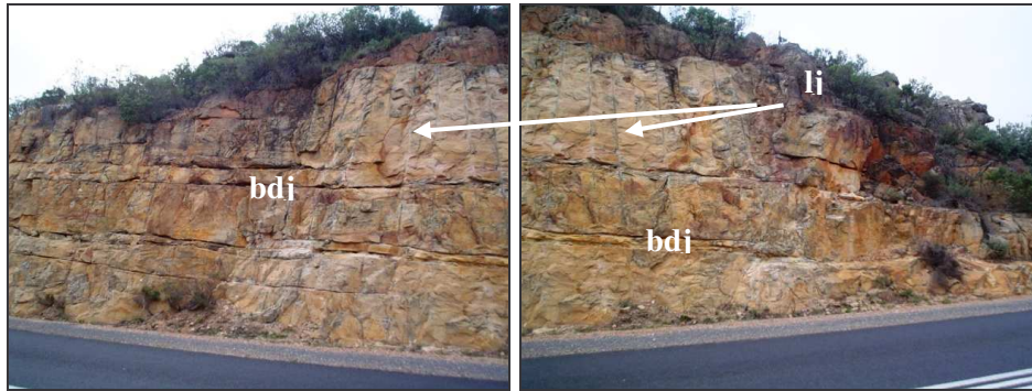
Figure 5.7 Panorama view of bedding planes in Peninsula Formation, near Graafwater.
