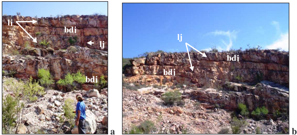
Figure 5.6 a & b Bedding and conjugate joints in Nardouw Subgroup, N7 near Algeria turnoff.
