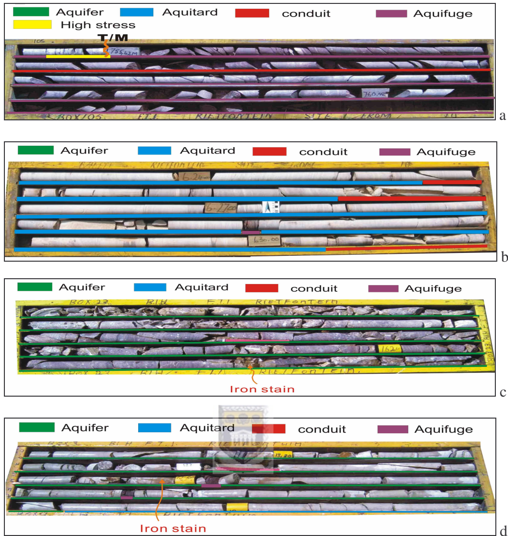
Figure 5.12a –d Core box 105 (a), 88(b), 23(c) &3(d) showing bed and conjugate joints at various depths.
