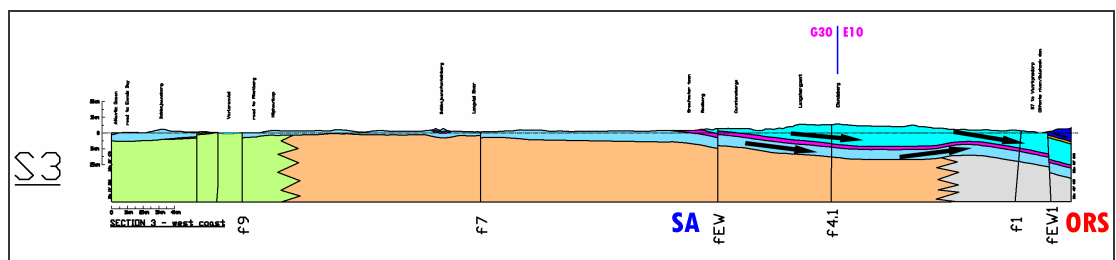
Figure 4.16 c Cross section 3 showing flow direction.
