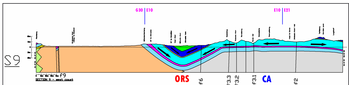
Figure 4.16 i Cross section 9 showing flow direction.
