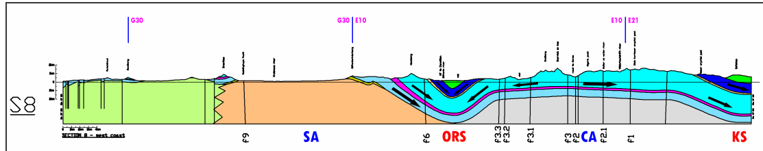
Figure 4.16 h Cross section 8 showing flow direction.
