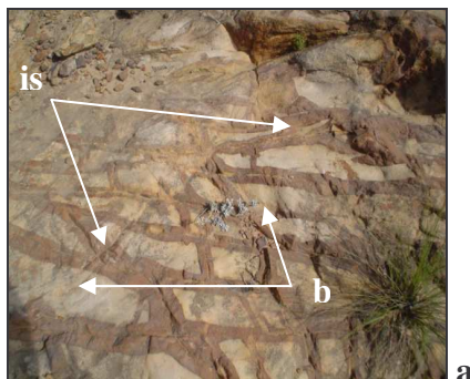
Figure 5.1a Blocky fault breccia
