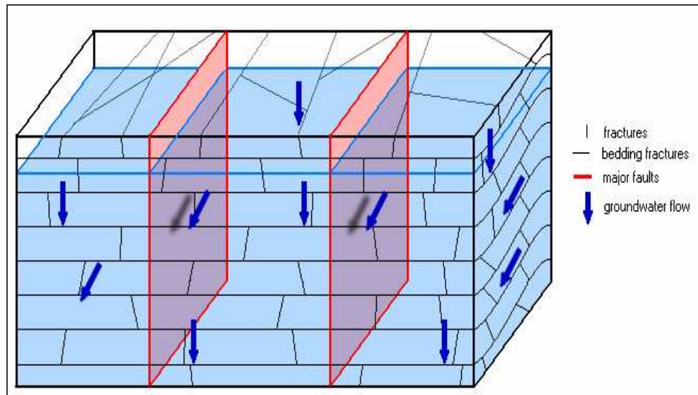
Figure 5.18 Conceptual flow in bedding and conjugate joints.
