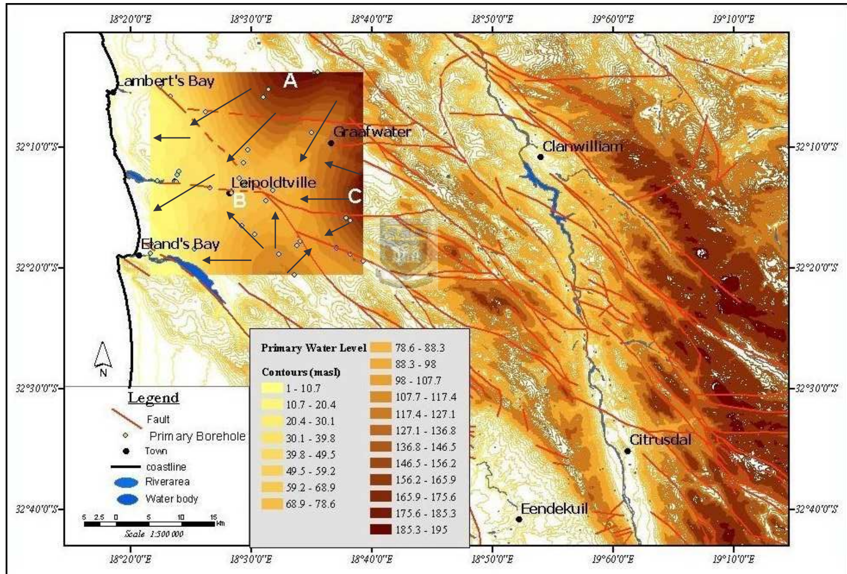
Figure 5.14 Water level contours for the Primary sand aquifer (using ordinary Kriging) Arrows indicate flow direction
