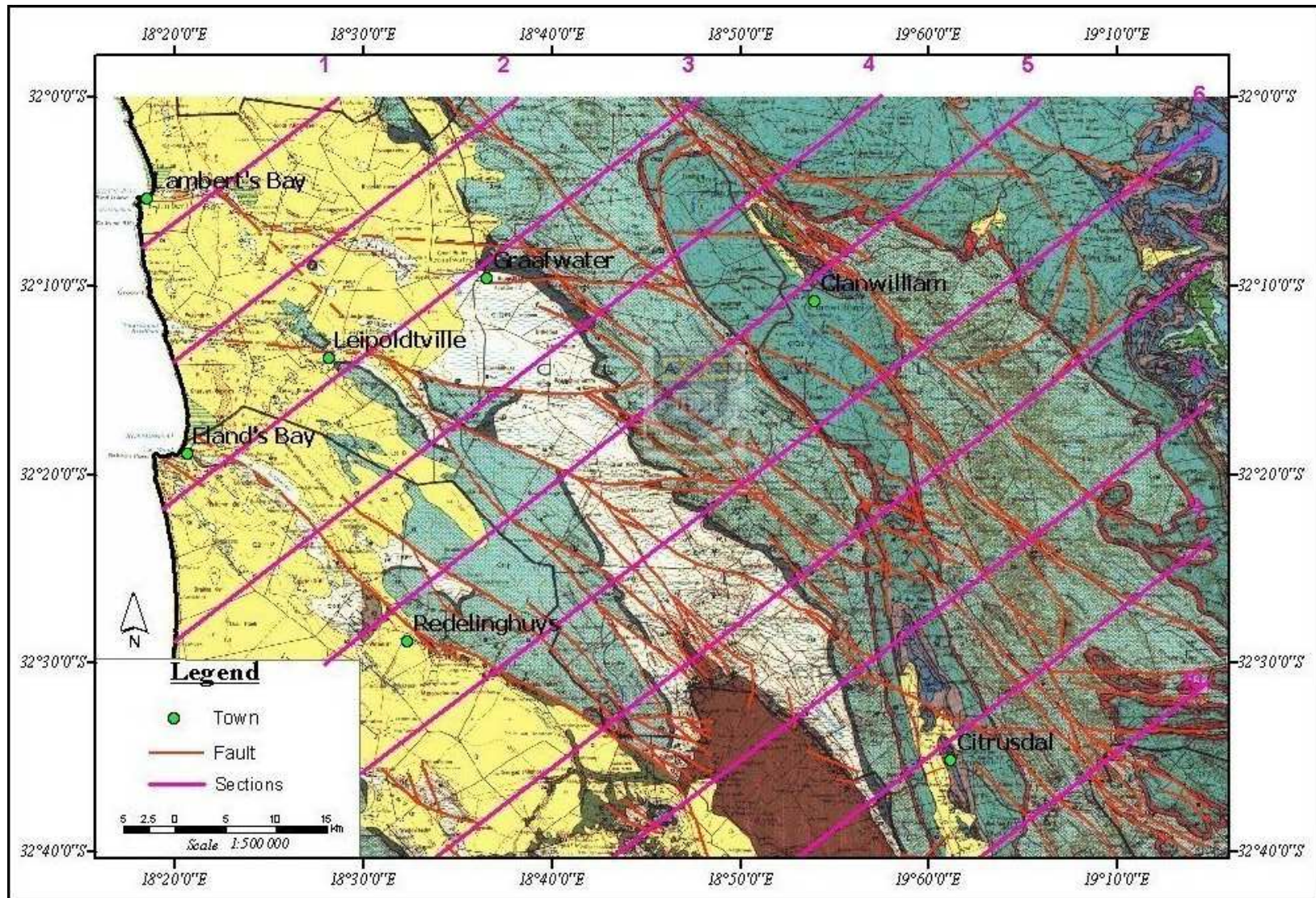
Figure 3.1 Position of cross section lines on geological map (based on published 1:250000 map,3218Clanwilliam,1973,Council For Geoscience)
