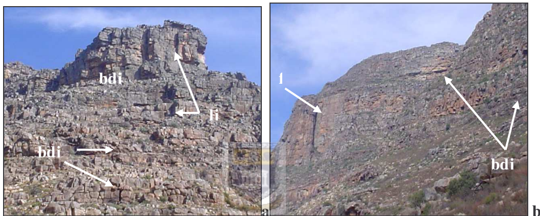
5.9 a & b Bedding and conjugate joints in Peninsula Formation, Cederberg Mountains.
