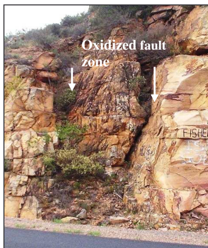
Figure 5.4 Open fault with oxidized zone, near Graafwater.
