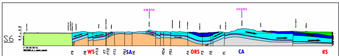
Figure 4.16 f Cross section 6 showing flow direction.
