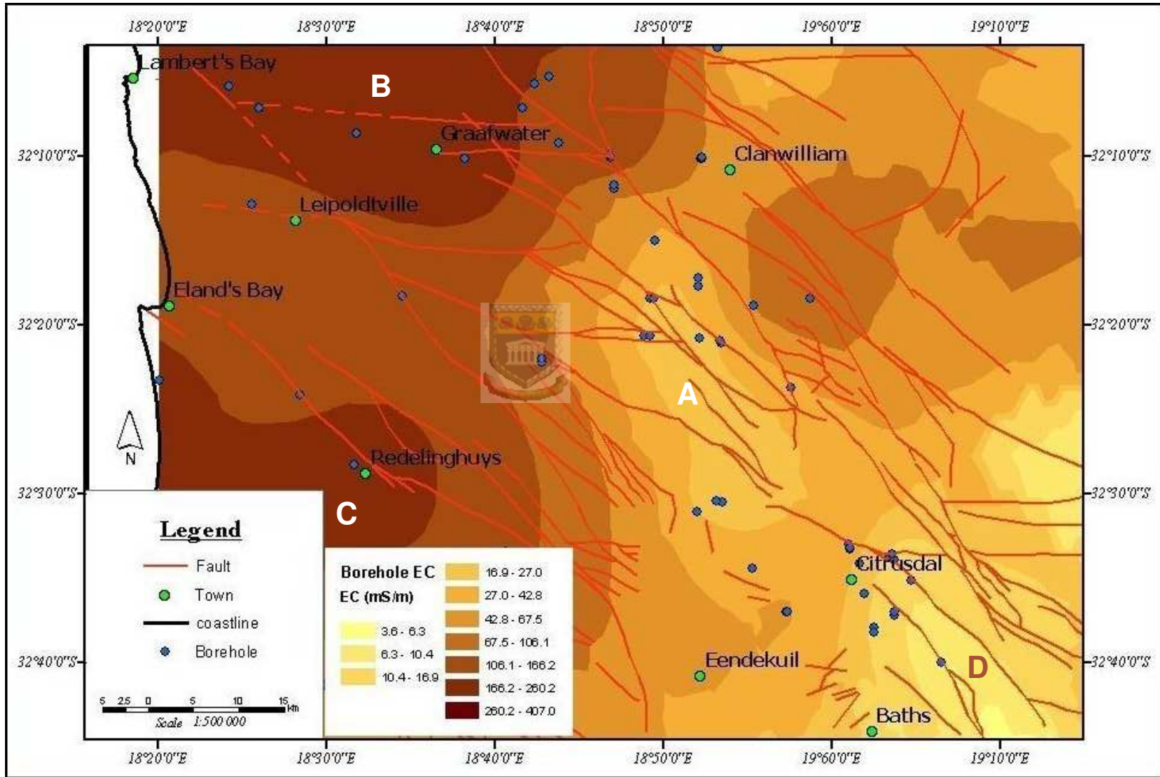
Figure5.15 EC value contours for the Secondary aquifer (using ordinary Kriging)
