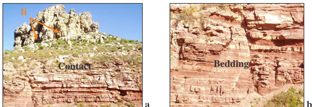
Figure 5.11 a & b Contact zone of Klipheuwel Formation under lying Piekenierskloof Formation, Elands Bay.
