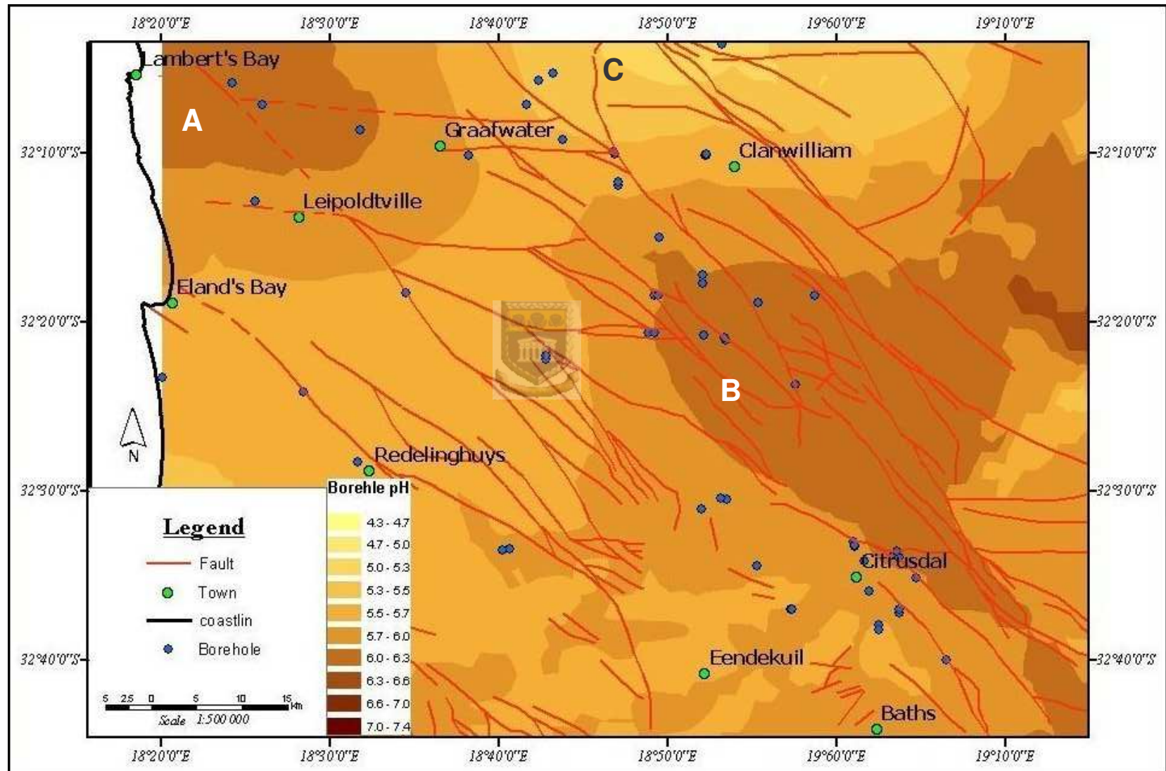
Figure 5.16 pH value contours for the Secondary aquifer ( using ordinary Kriging)
