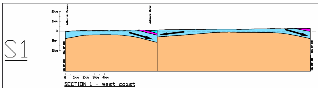
Figure 4.16 a Cross section 1 showing flow direction.
