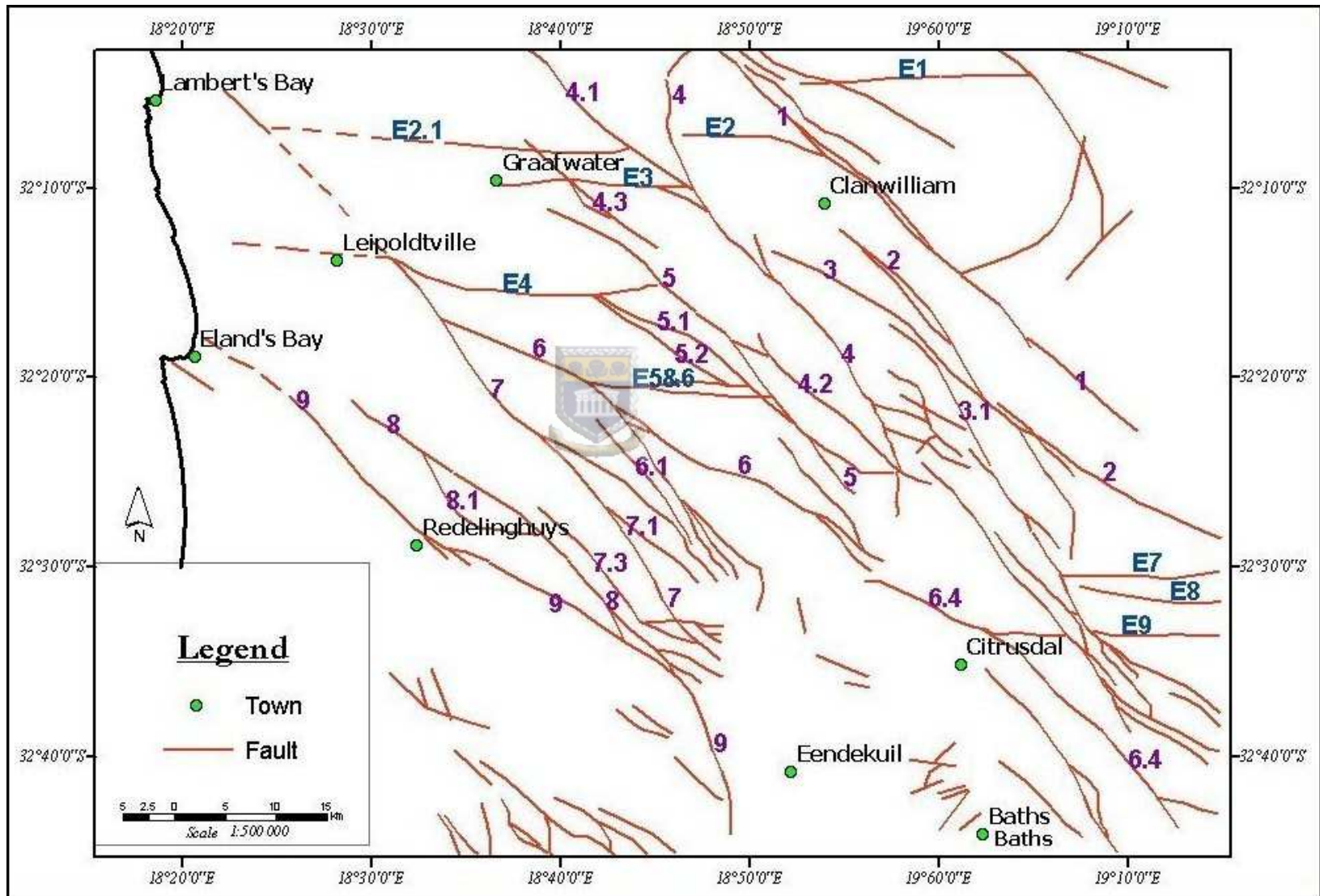
Figure 4.13 Numbered main faults of study area, with northwesterly faults(purple) and easterly faults(blue)
