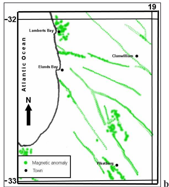
Figure 4.10b Aeromagnetic survey anomalies, (modified from Umvoto/SRK 2000).
