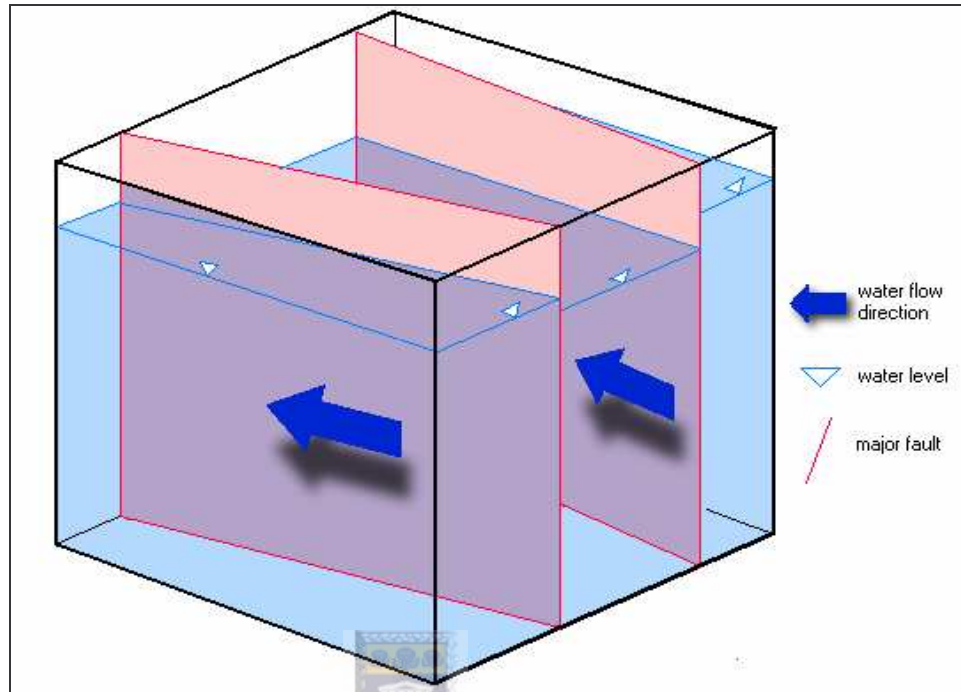
Figure 3.4 Flow between faults
