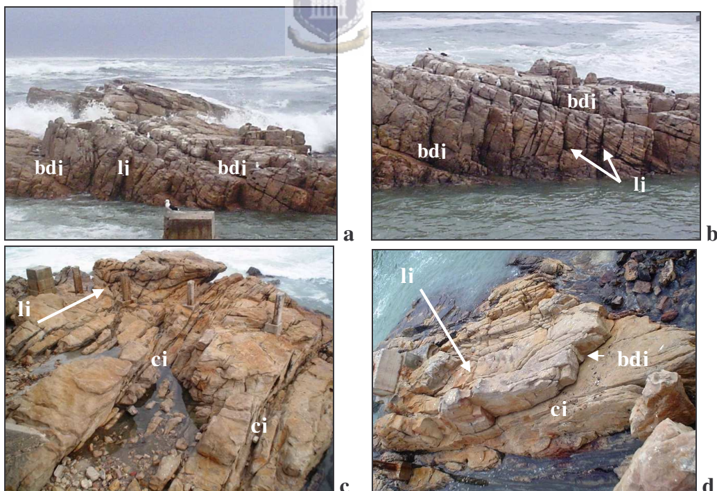
5.8 a, b, c & d Bedding, long and cross joints in Piekenierskloof Formation, Lambert's Bay.
