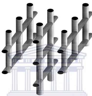
Figure 2-6: Tubular schematic of the two-dimensional channel system of Gismondine-type structures (Gottardi and Galli, 1985).
