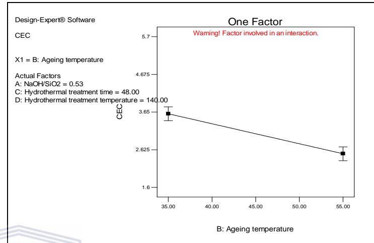
Figure 4-36: Main effect of ageing temperature.
