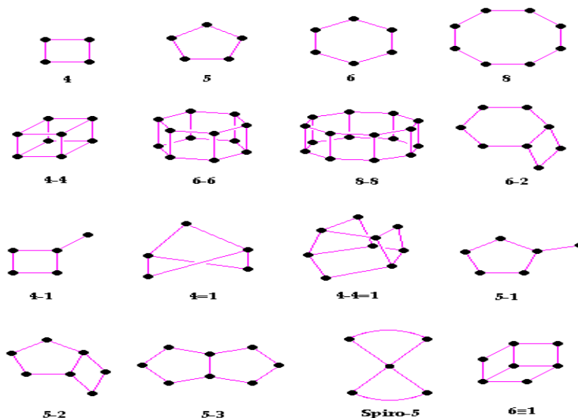
Figure 2-4: Secondary building units; the corner of the polyhedra represent tetrahedral atoms (Nagy et al. , 1998).
