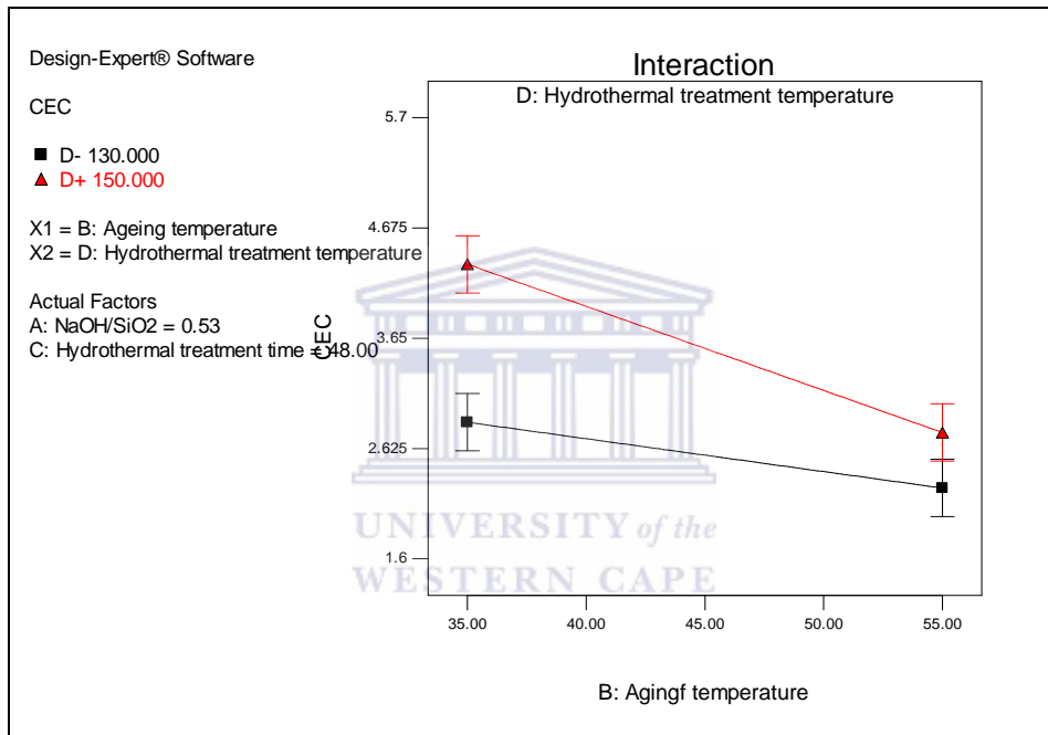
Figure 4-40: Interaction between ageing and hydrothermal treatment temperature.
