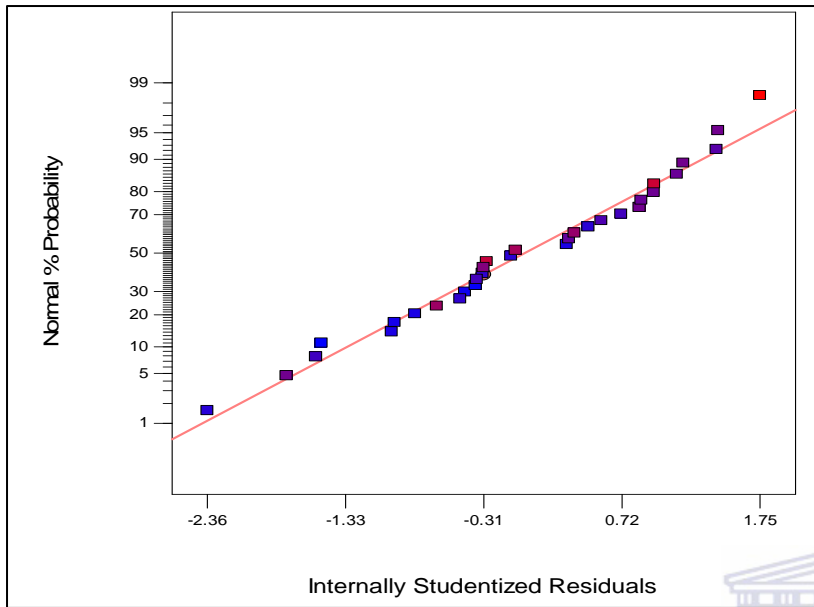
Figure 4-28: Normal plot of residuals.
