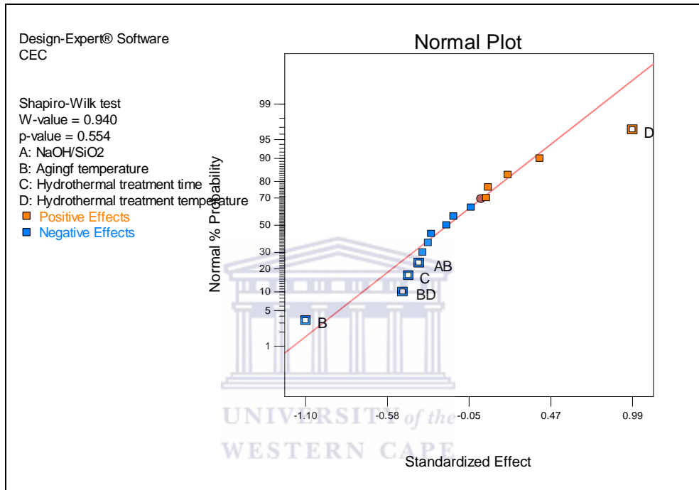
Figure 4-27: Normal probability plot.
