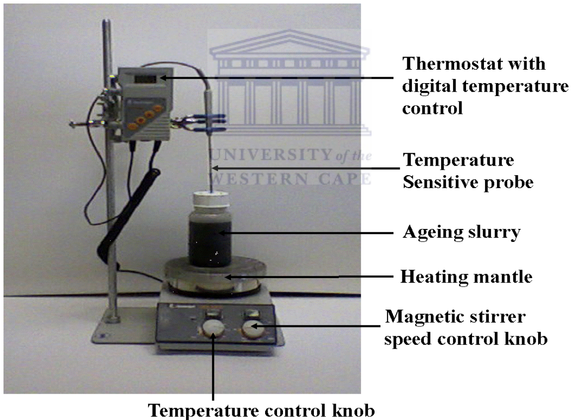
Figure 3-2: Experimental set-up during ageing process.
