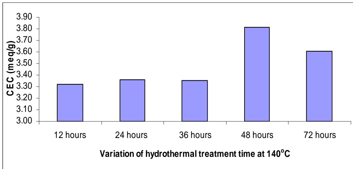
Figure 4-23: Effect of variation of hydrothermal treatment time on cation exchange capacity.
