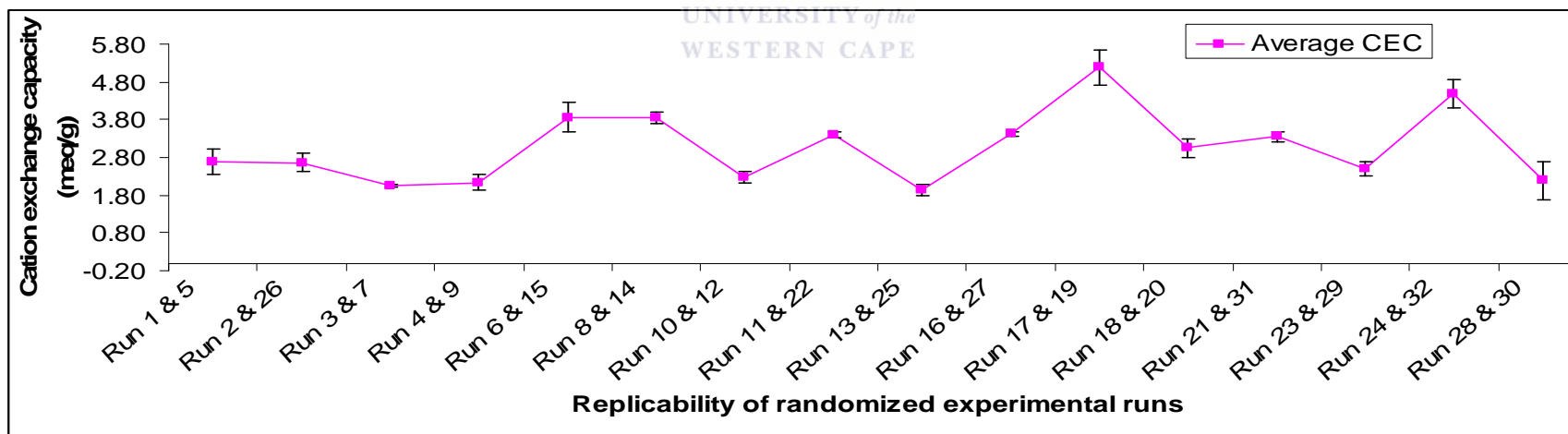
Figure 4-26: Replicability of designed experiments (Error bars represents standard error of average cation exchange capacity).
