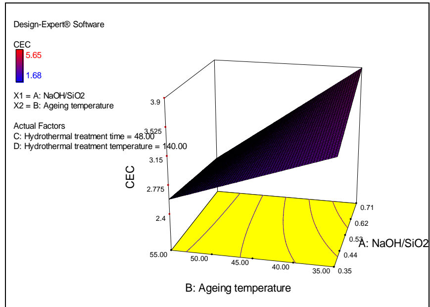
Figure 4-41: Three-dimensional response surface (relationship between ageing temperature and NaOH/SiO 2 molar ratio)
