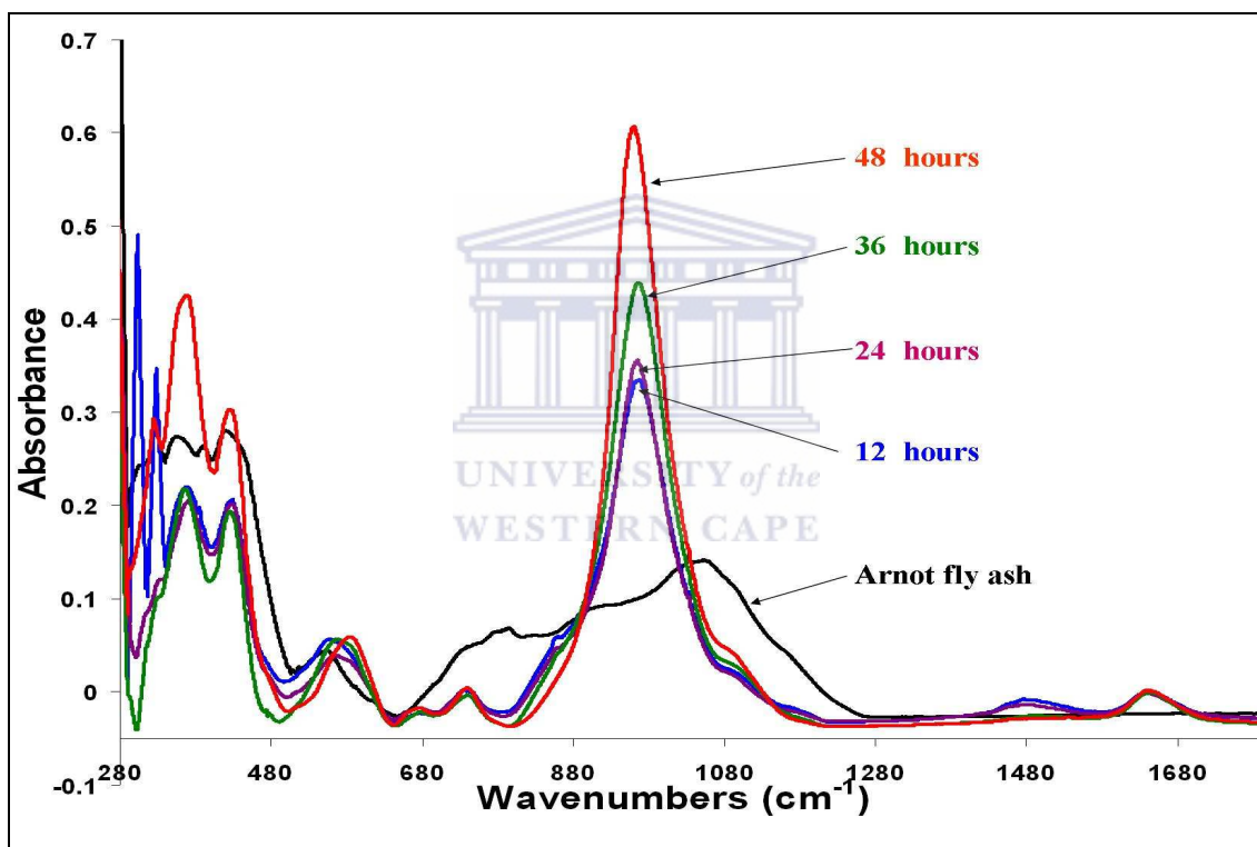
Figure 4-14: FT-IR spectra of zeolites synthesized at 140\text{ }^{\circ}\text{C} by varying time of hydrothermal treatment.
