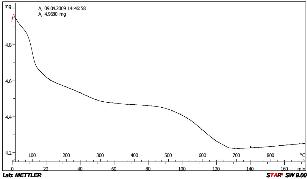
Figure 4-21: Weight-temperature behaviour of zeolite Na-P1 by TGA.
