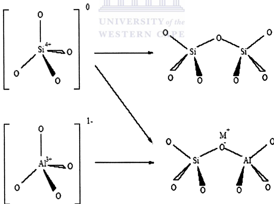
Figure 2-2: Primary building blocks of zeolites.
