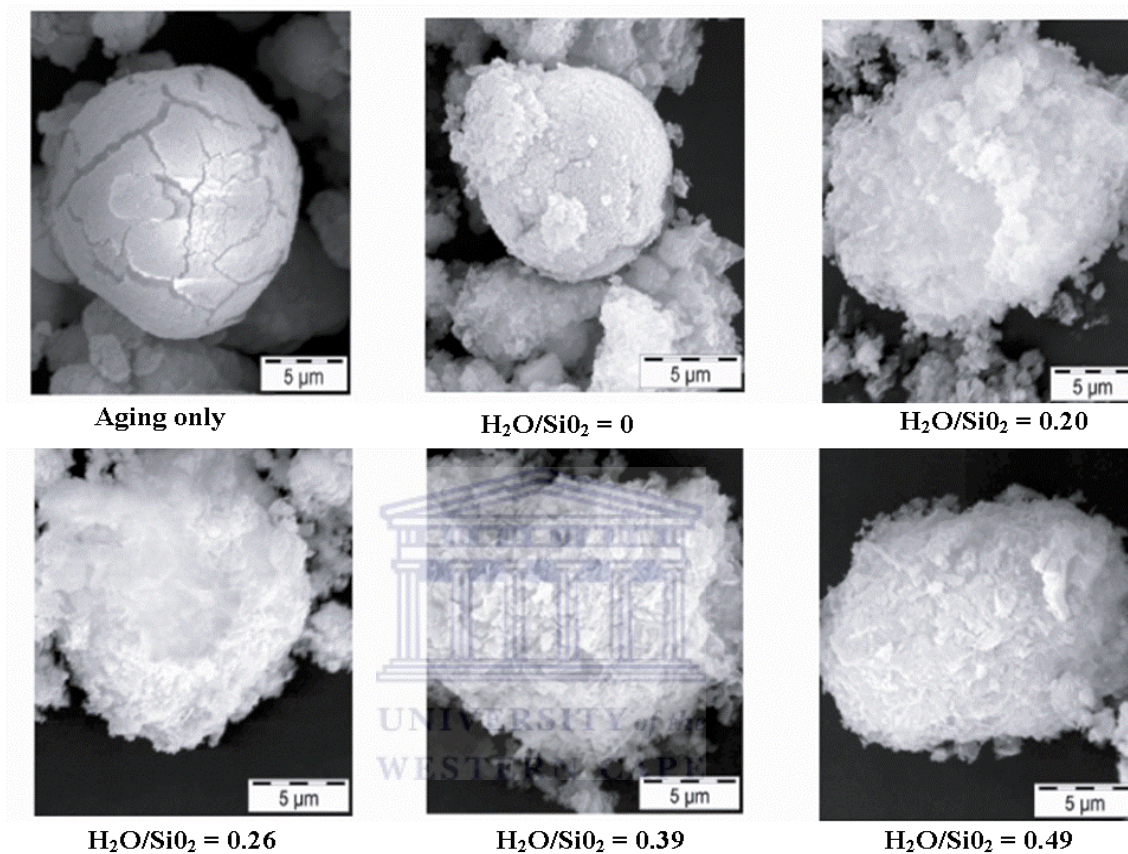
Figure 4-17: SEM images showing the products obtained with variation of water content during the hydrothermal treatment process.
