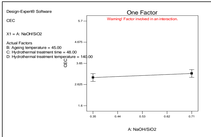
Figure 4-35: Main effect of NaOH/SiO 2 molar ratio.
