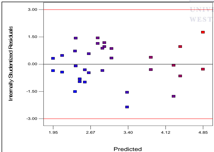
Figure 4-30: Plot of residuals versus predicted
