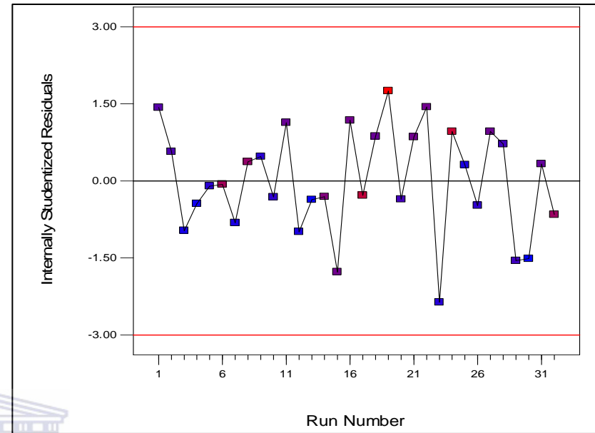
Figure 4-29: Plot of Residuals versus runs.
