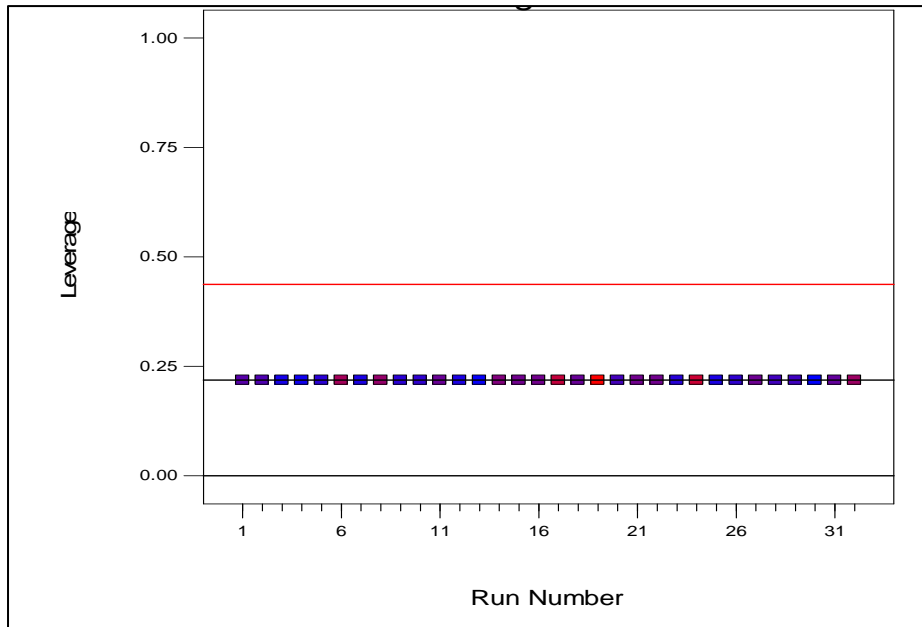
Figure 4-33: Plot of leverage versus run.
