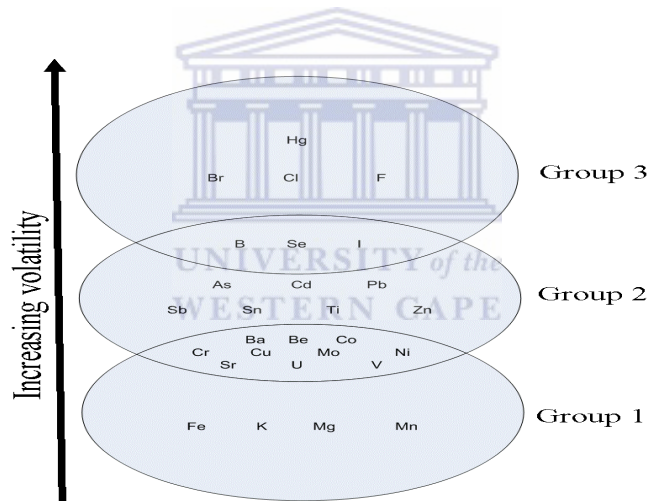
Figure 2-1: Classification of trace elements in coal combustion by-products by their relative volatility (Vories and Thogmorton, 2002).
