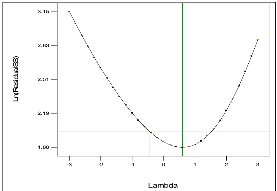
Figure 4-32: Box-Cox plot for power transforms.
