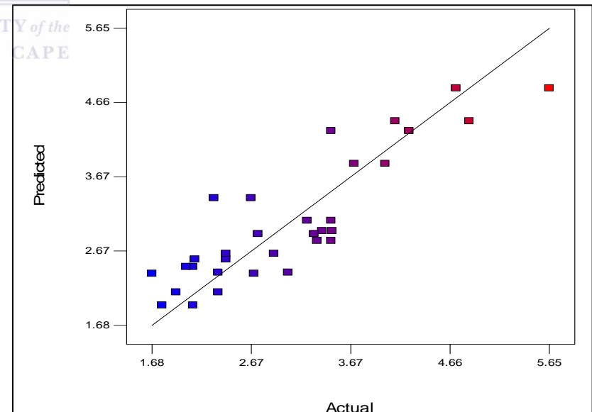
Figure 4-31: Plot of predicted versus actual.
