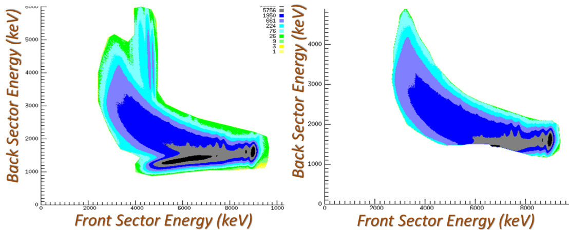
(A) Banana spectra for sectors before banana gates are done
