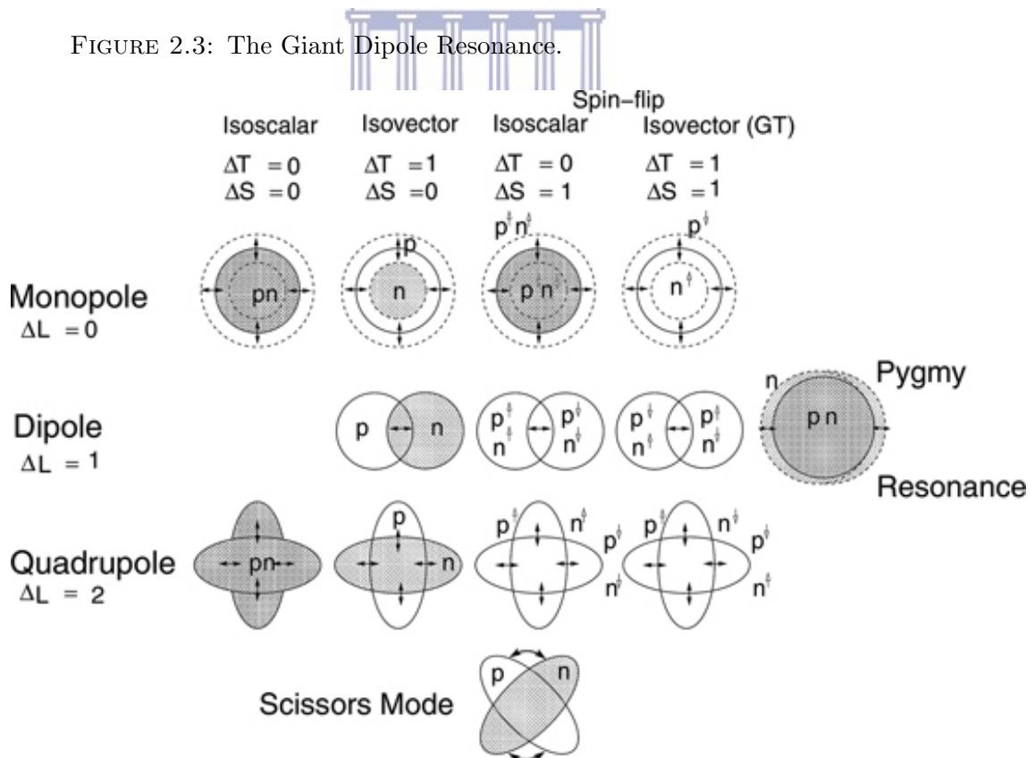
FIGURE 2.4: A qualitative scheme of giant resonance modes of the nucleus, courtesy of [12].
