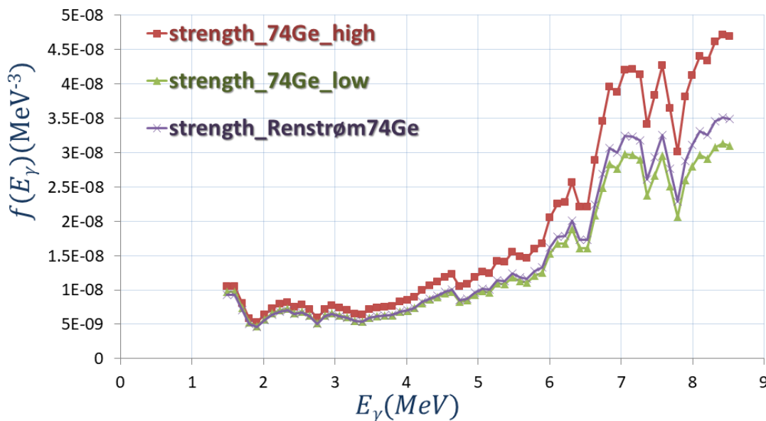
FIGURE 5.6: A plot of the data from the reaction {}^{74}\text{Ge}({}^3\text{He}, {}^3\text{He}^*){}^{74}\text{Ge} , taken from Ref [3]. The actual data on the plot are represented by the purple line, the red line is the upper uncertainty limit and the green one is the lower uncertainty limit.
