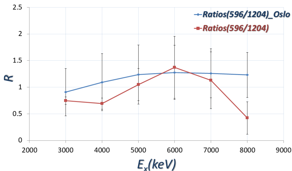
FIGURE 5.8: A plot of the data from figure 5.3 in brown and the Oslo data in blue rebinned with the use of a polynomial fit of order 2.
