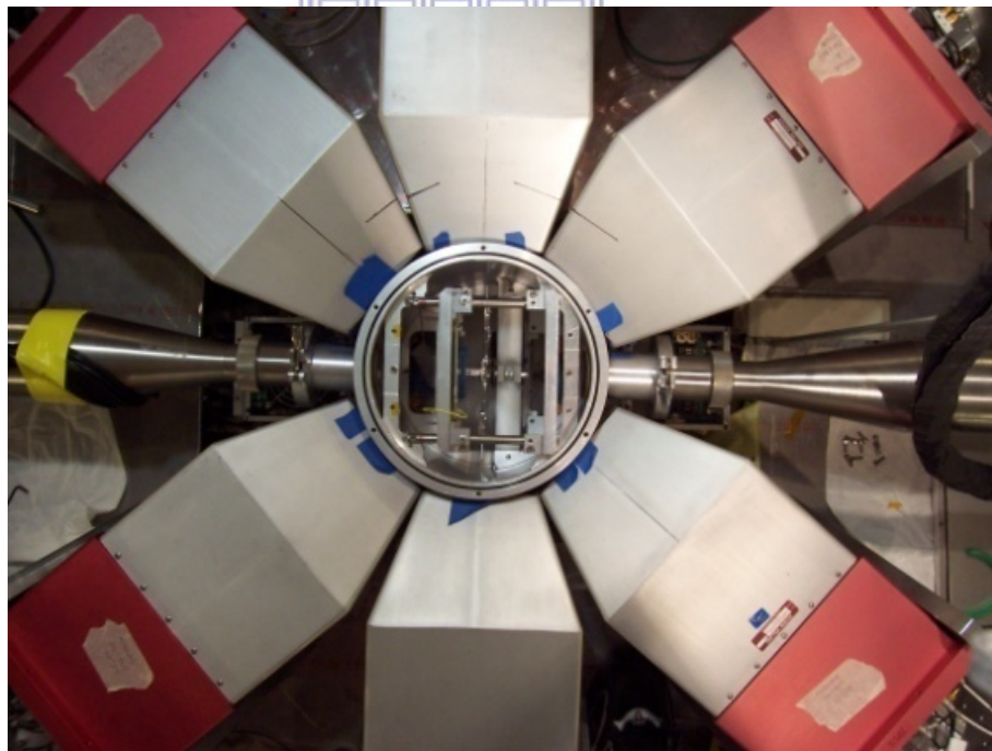
FIGURE 3.1: The clover detectors used for \gamma -ray detection [24].
