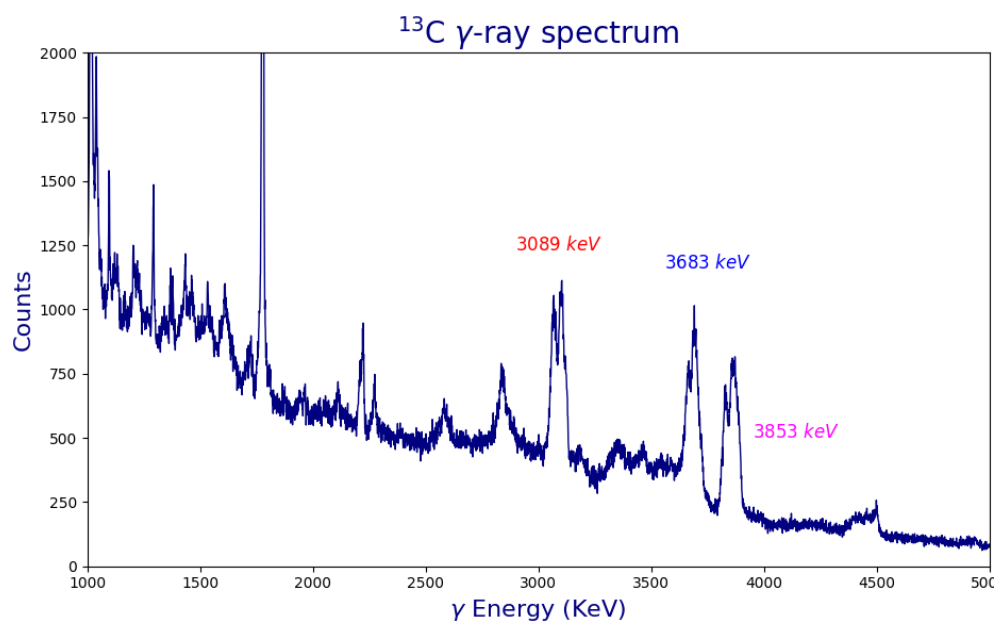
FIGURE 4.18: Three \gamma -rays that were used for efficiency calibration coming from ^{13}\text{C} .
