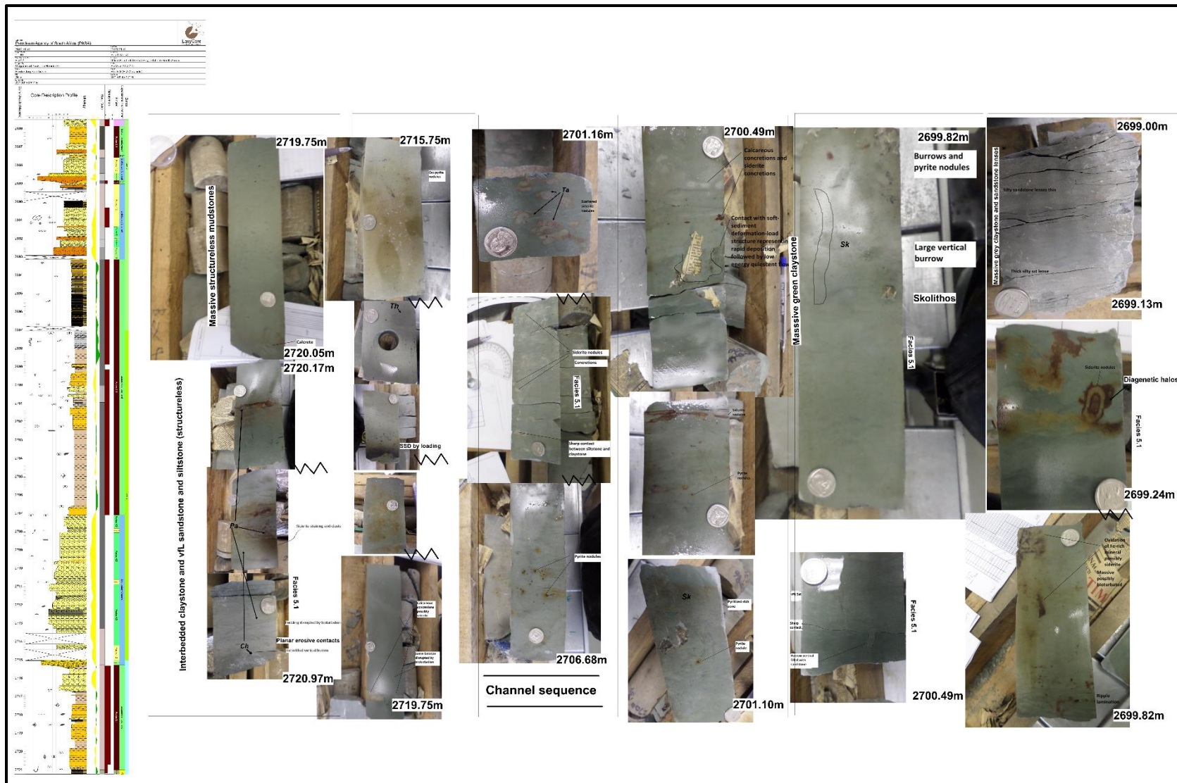
Figure 4.1.10: Examples of facies association 5 showing offshore transgressive or embayment mudstones. Trace fossils consisted of chondrites (Ch), Skolithos (Sk), Paleophycus (Pa), Thalassinoides (Th), Taenidium (Ta) and cryptically bioturbated structures (fine matrix). Pyrite and siderite nodules and staining are common.
